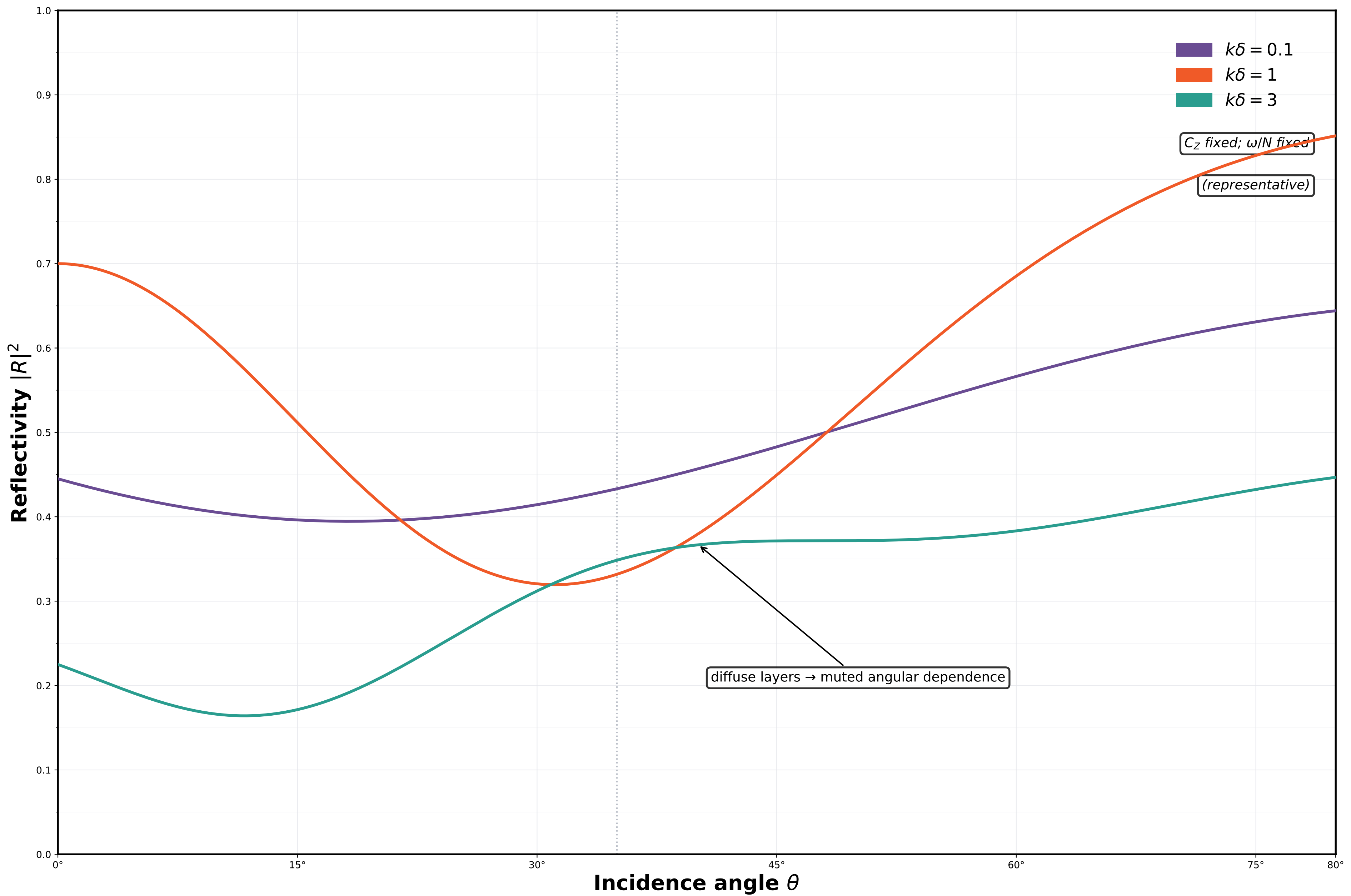
Figure 3.5C. Reflectivity vs incidence for thickness parameter k\delta at fixed contrast. Thin/sharp layers yield pronounced obliquity-dependent lobes; diffuse layers produce smoother, muted trends.
