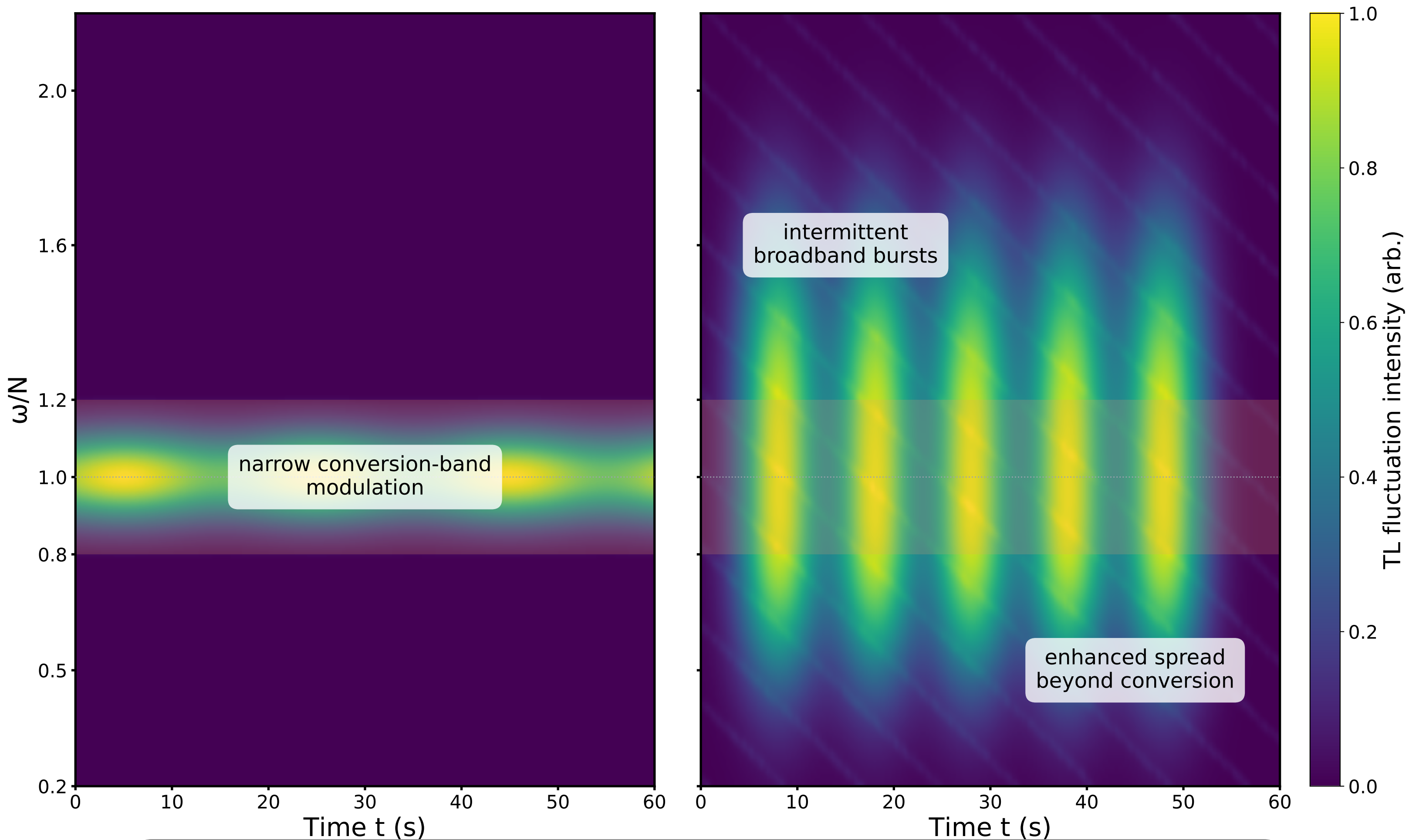
Figure 3.6B — Time-frequency TL fluctuation intensity
