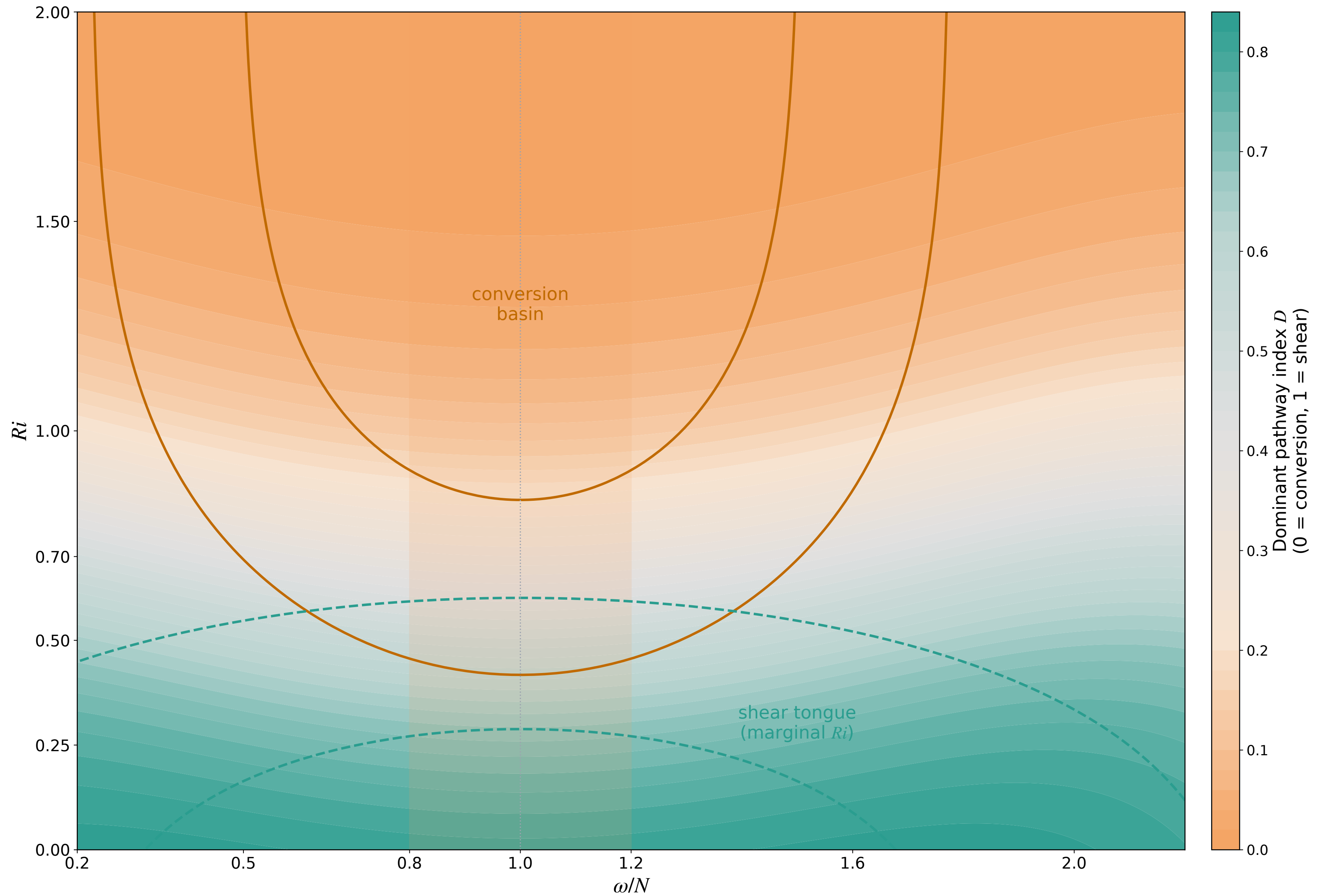
Figure 3.8A. Predicted dominant pathway map for continuous stratification. Conversion dominates near \omega/N \approx 1 at higher Ri ; shear dominates under marginal Ri , especially around the conversion band.
