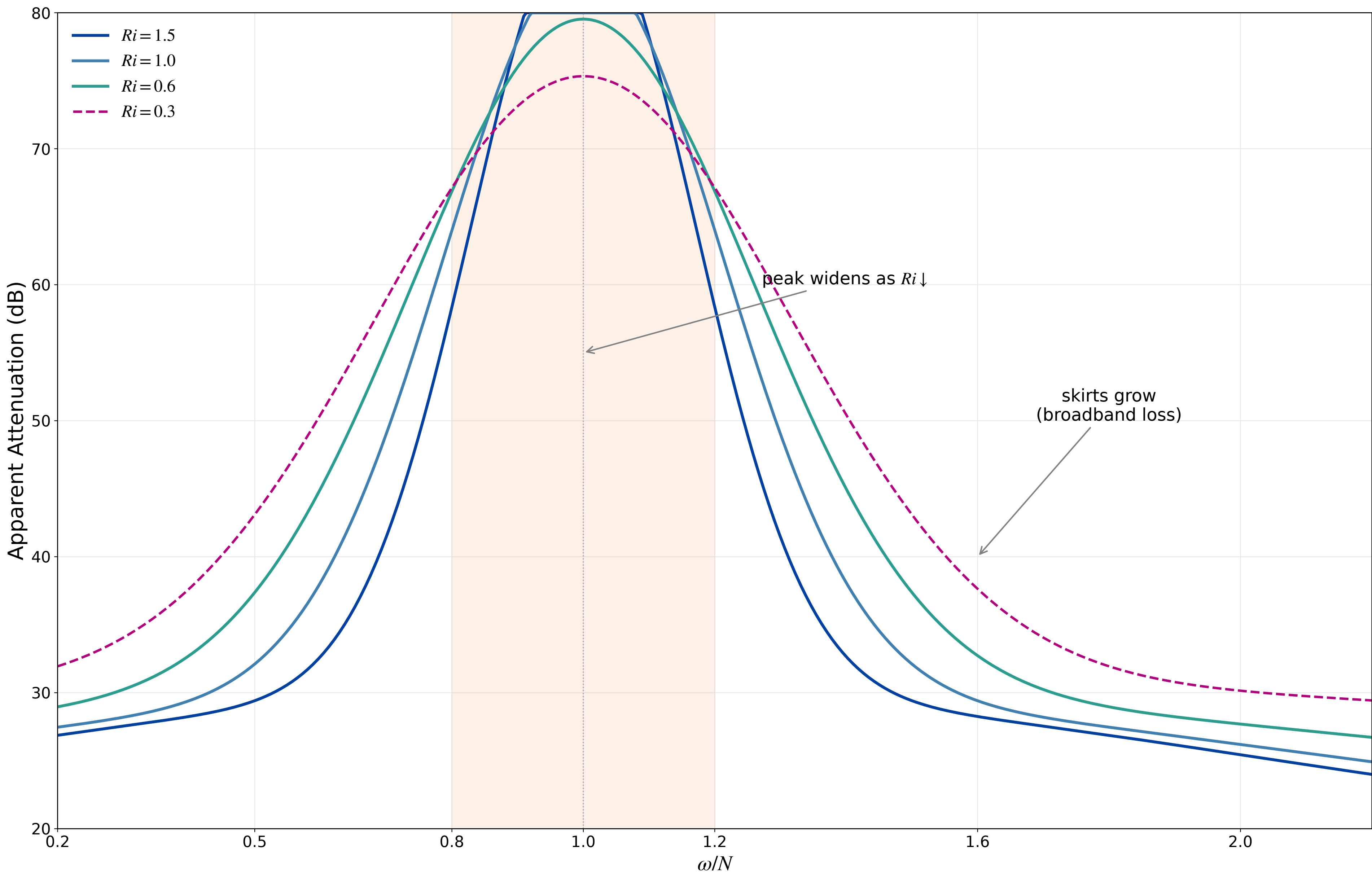
Figure 3.8C. Apparent attenuation vs \omega/N for selected Ri . Decreasing Ri broadens the conversion peak and raises broadband skirts.
