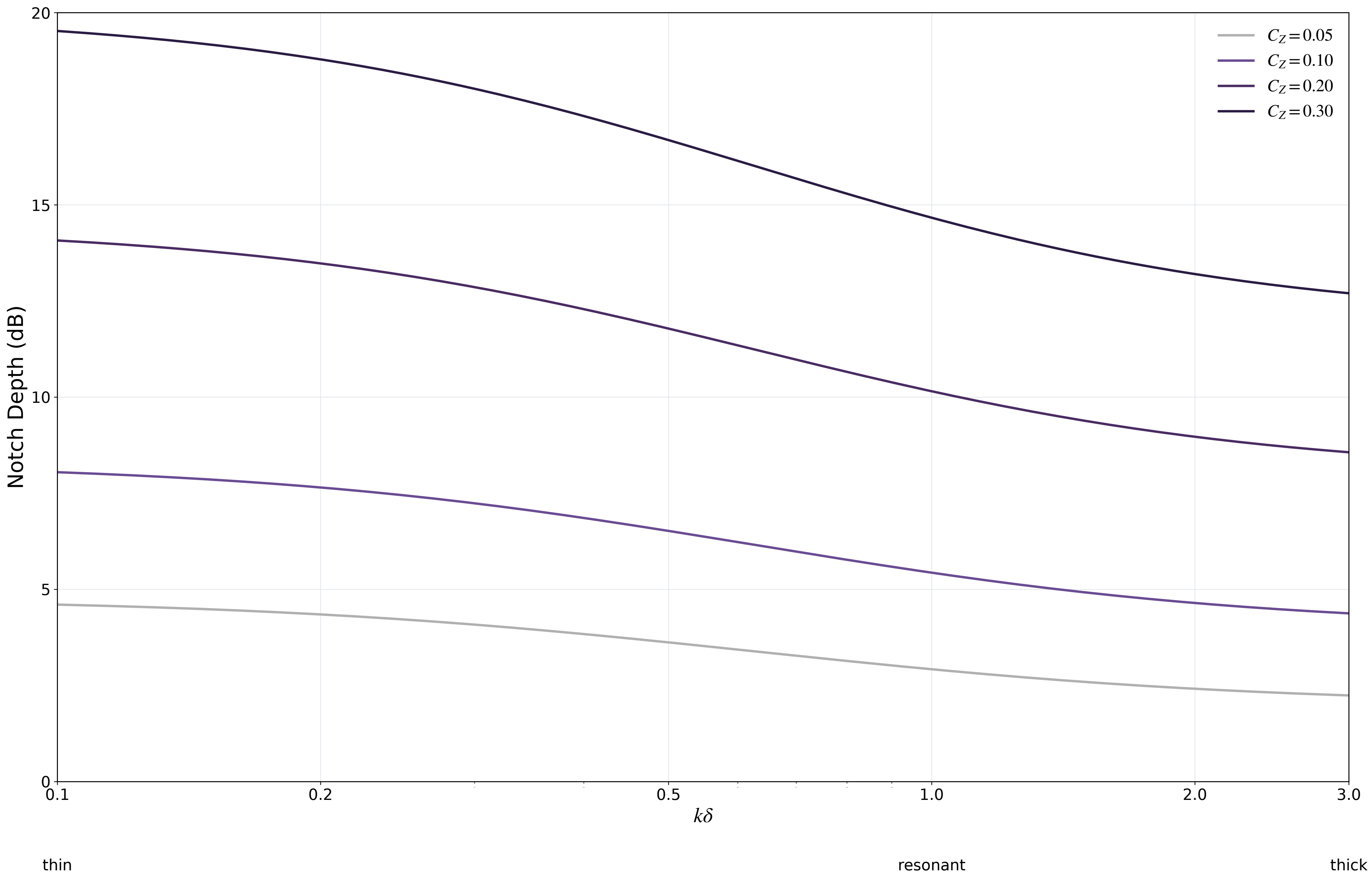
Figure 3.8D. Notch depth decreases as interface thickness k\delta increases and increases with impedance contrast C_Z .
