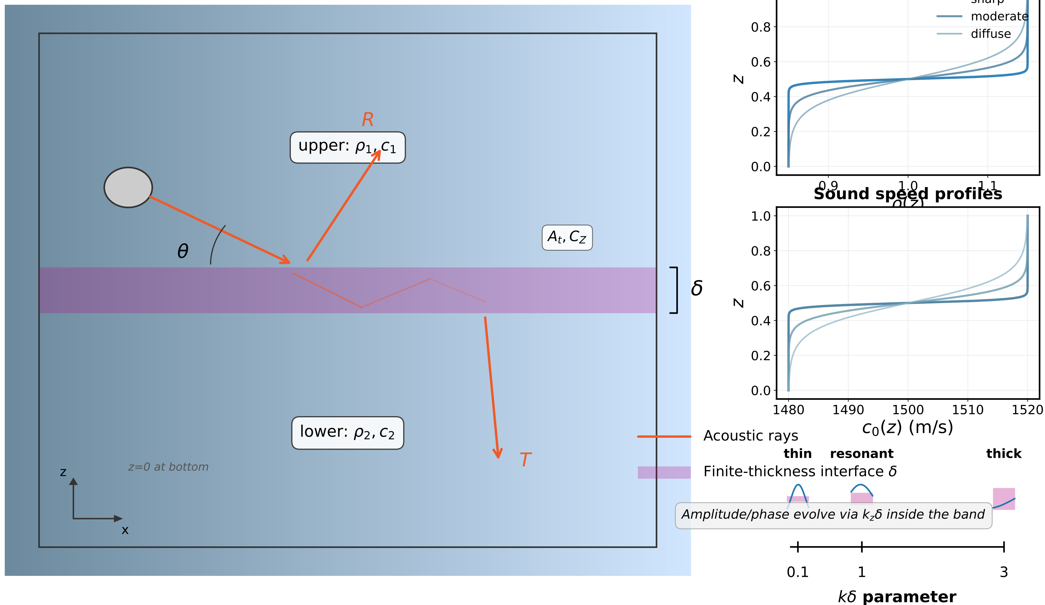
Figure 3.5A. Geometry of a finite-thickness interface with contrast (A_t, C_z) , incidence \theta , and phase-thickness k_z\delta . Multiple internal traversals generate frequency- and angle-dependent R/T .
