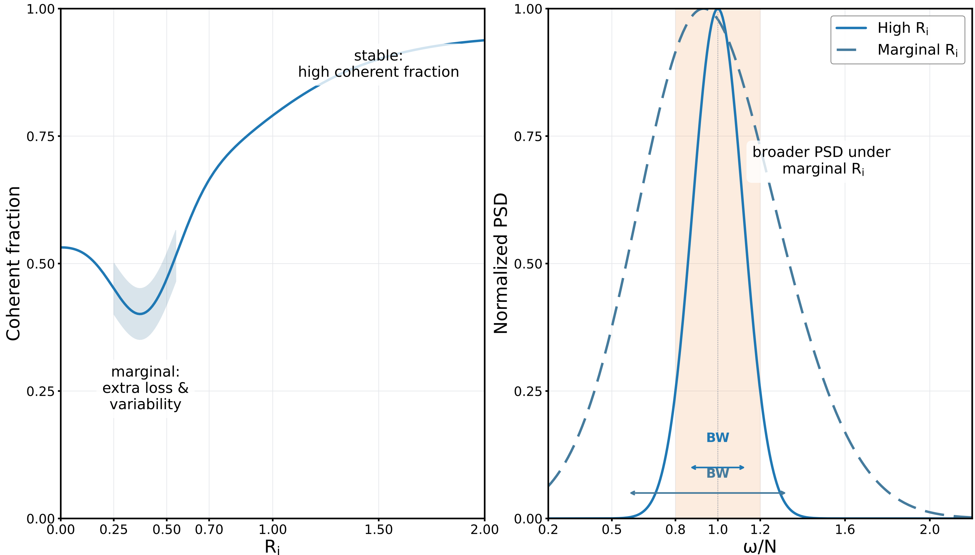
Figure 3.6C — Coherence loss and spectral broadening with decreasing R_i
