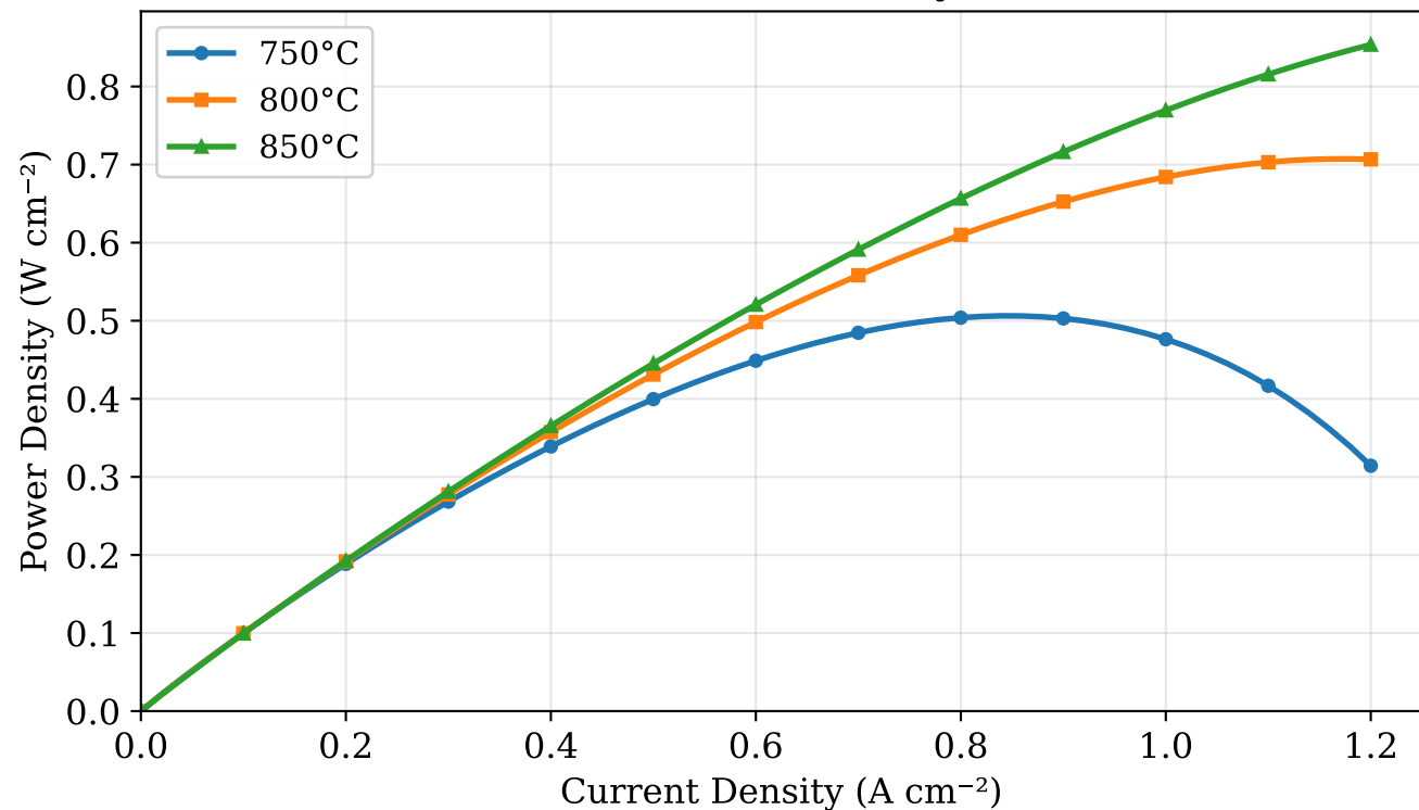
(b) Power Density
