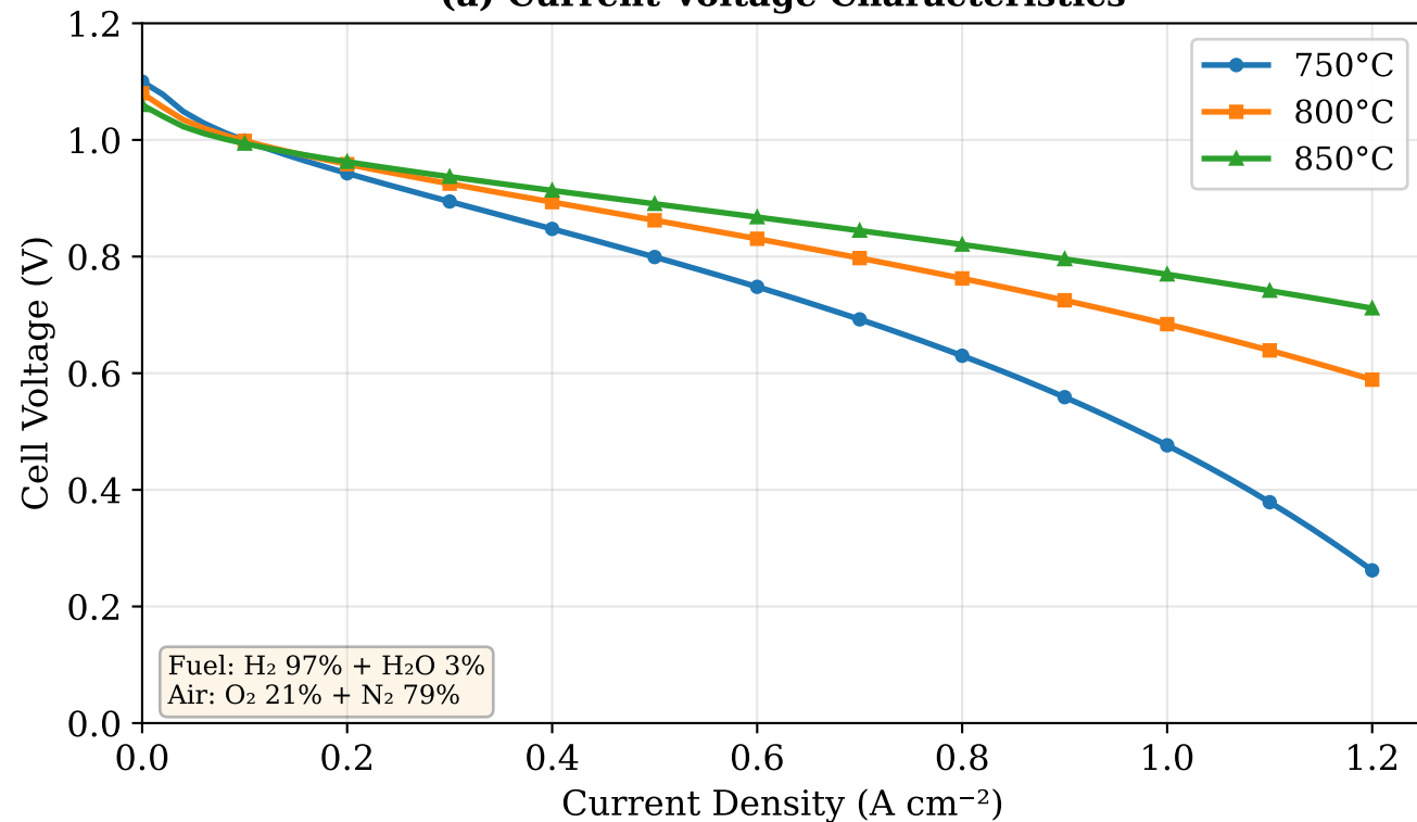
(a) Current-Voltage Characteristics
