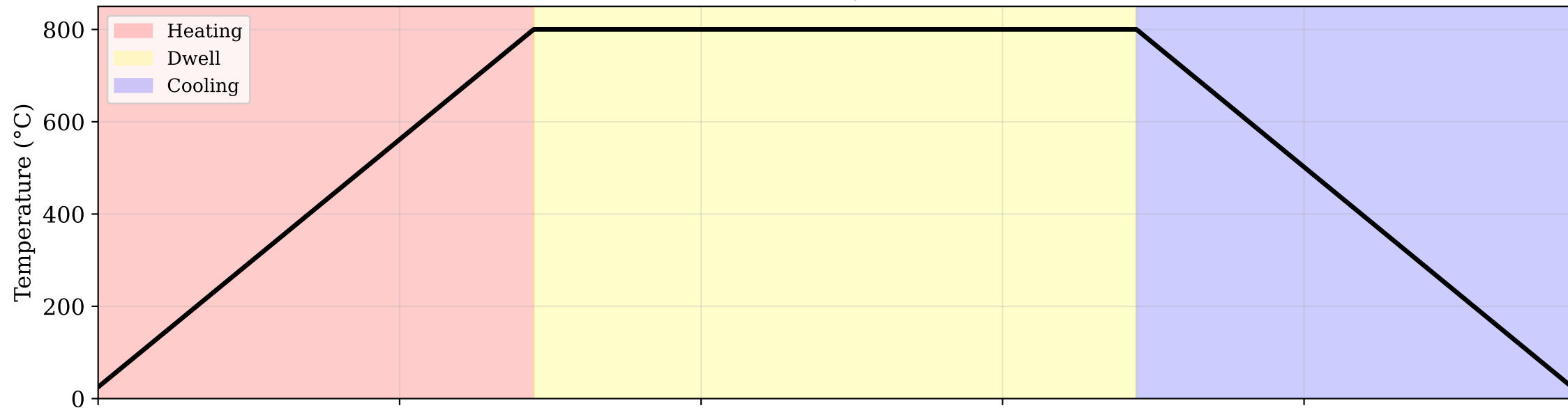
(a) Thermal Cycle Profile
