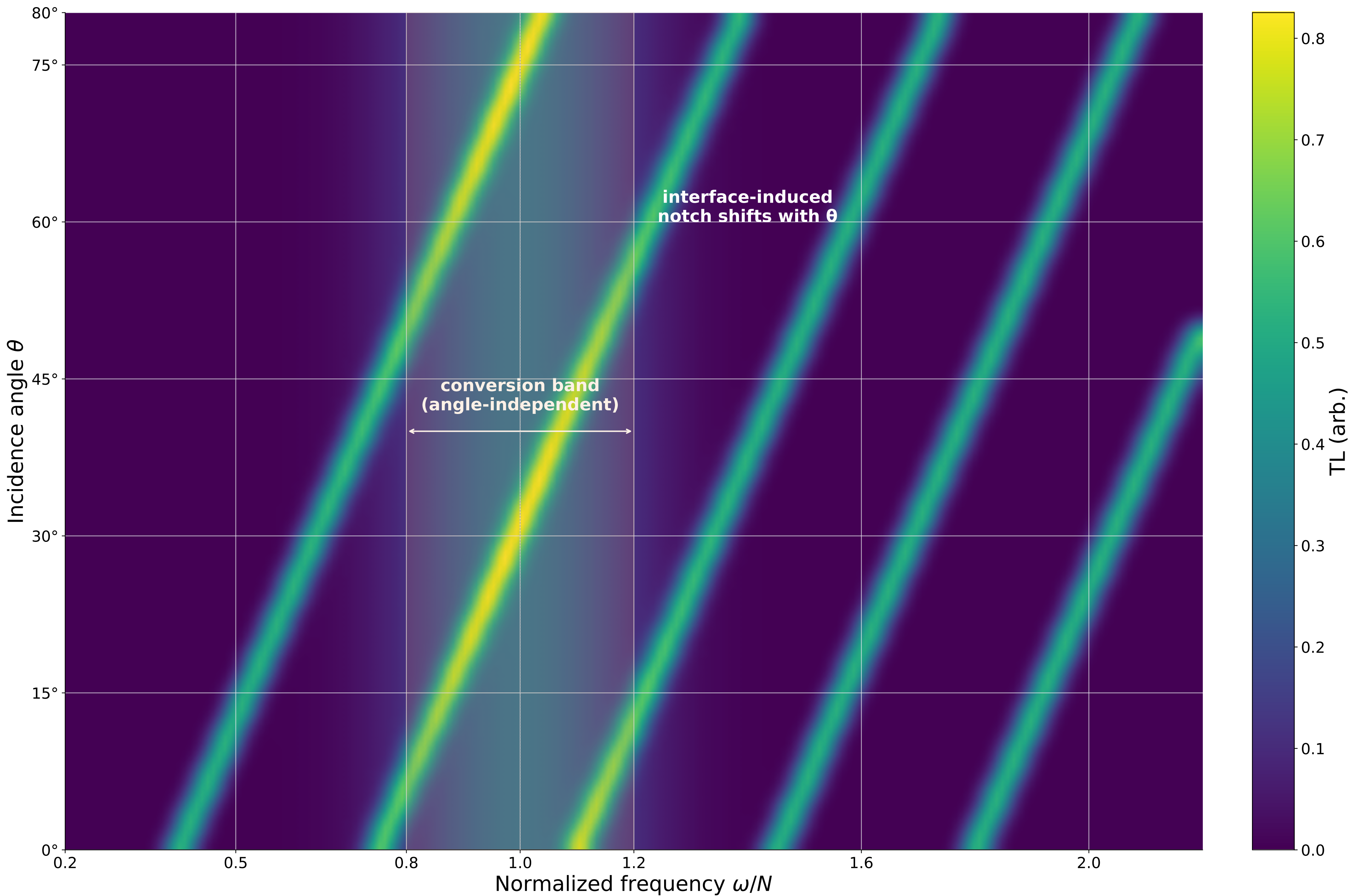
Figure 3.9B. Angle-frequency plate: interface-induced notches shift with angle, while the conversion band remains centered at \omega/N \approx 1 .
