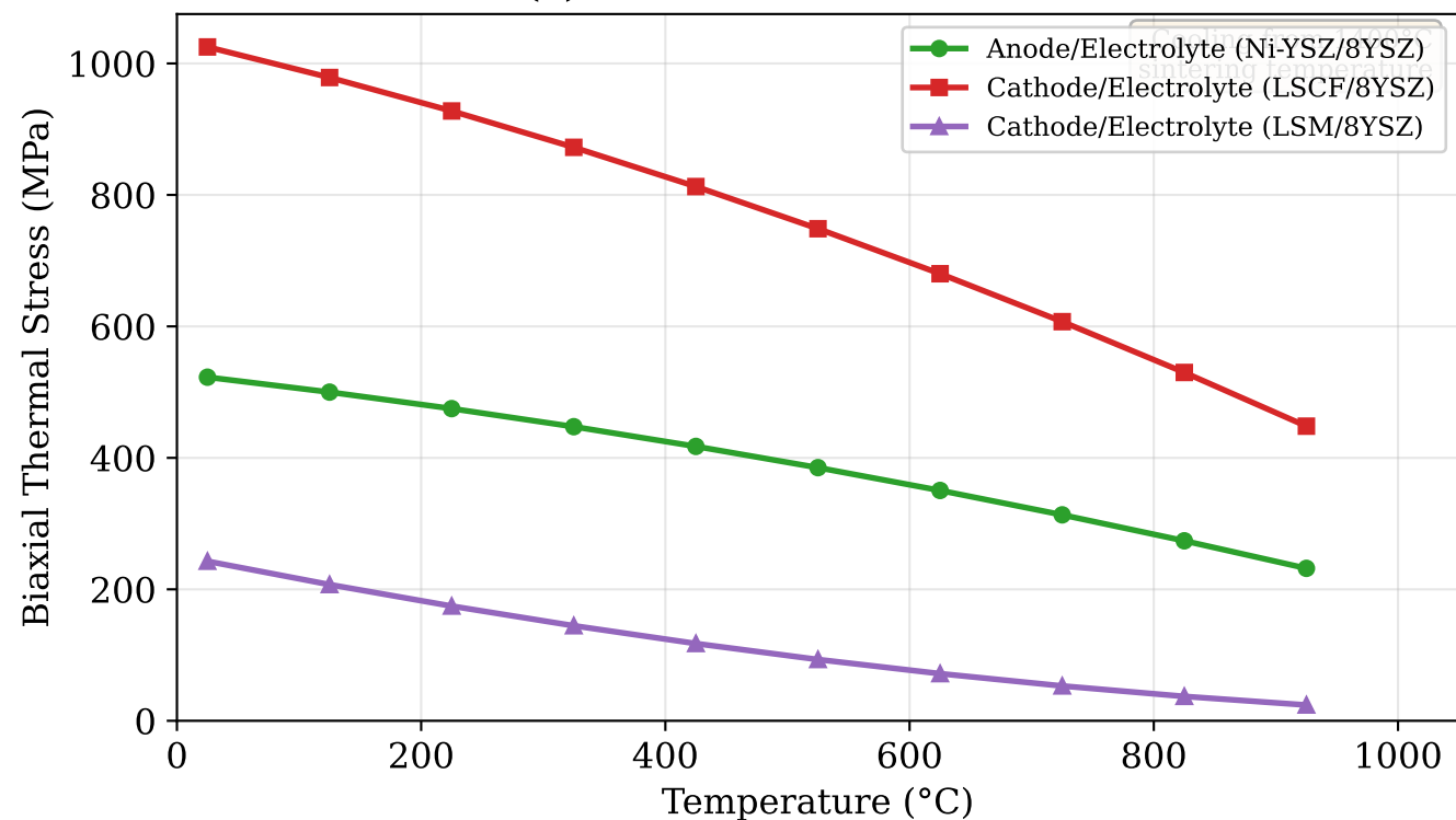
(b) Interfacial Thermal Stress
