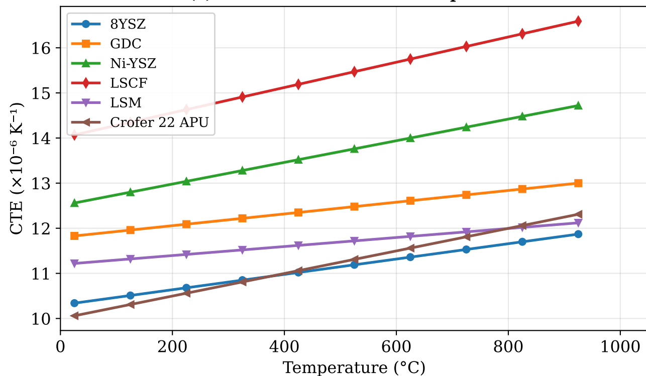
(a) Coefficient of Thermal Expansion
