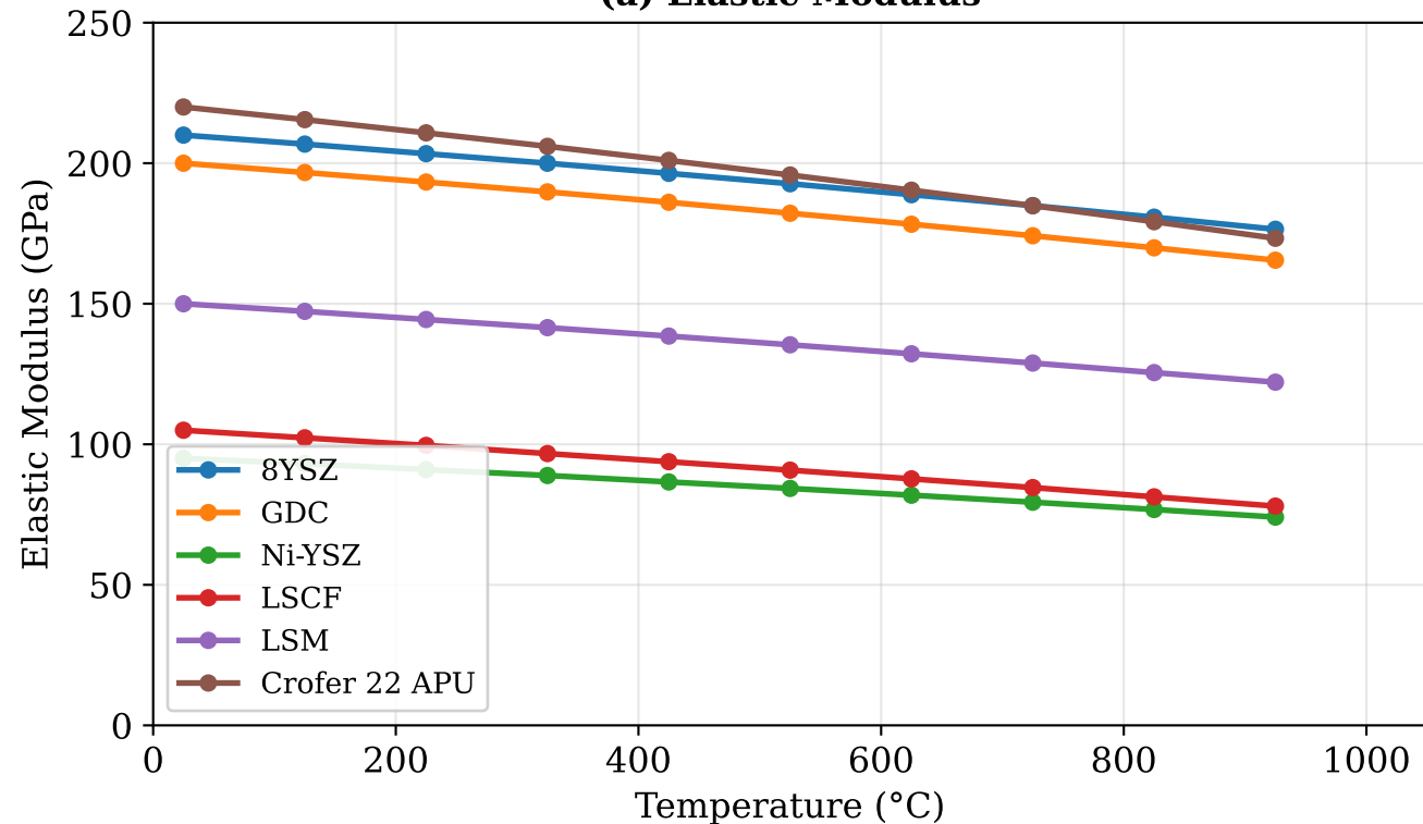
(a) Elastic Modulus
