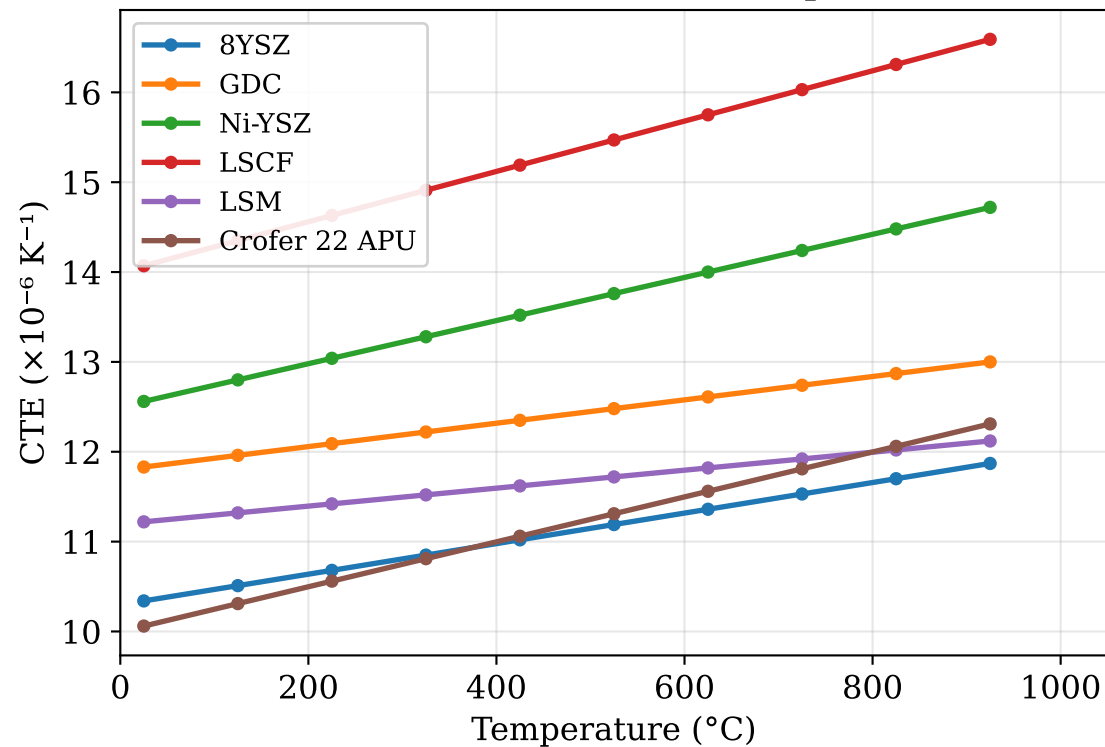
(a) Coefficient of Thermal Expansion
