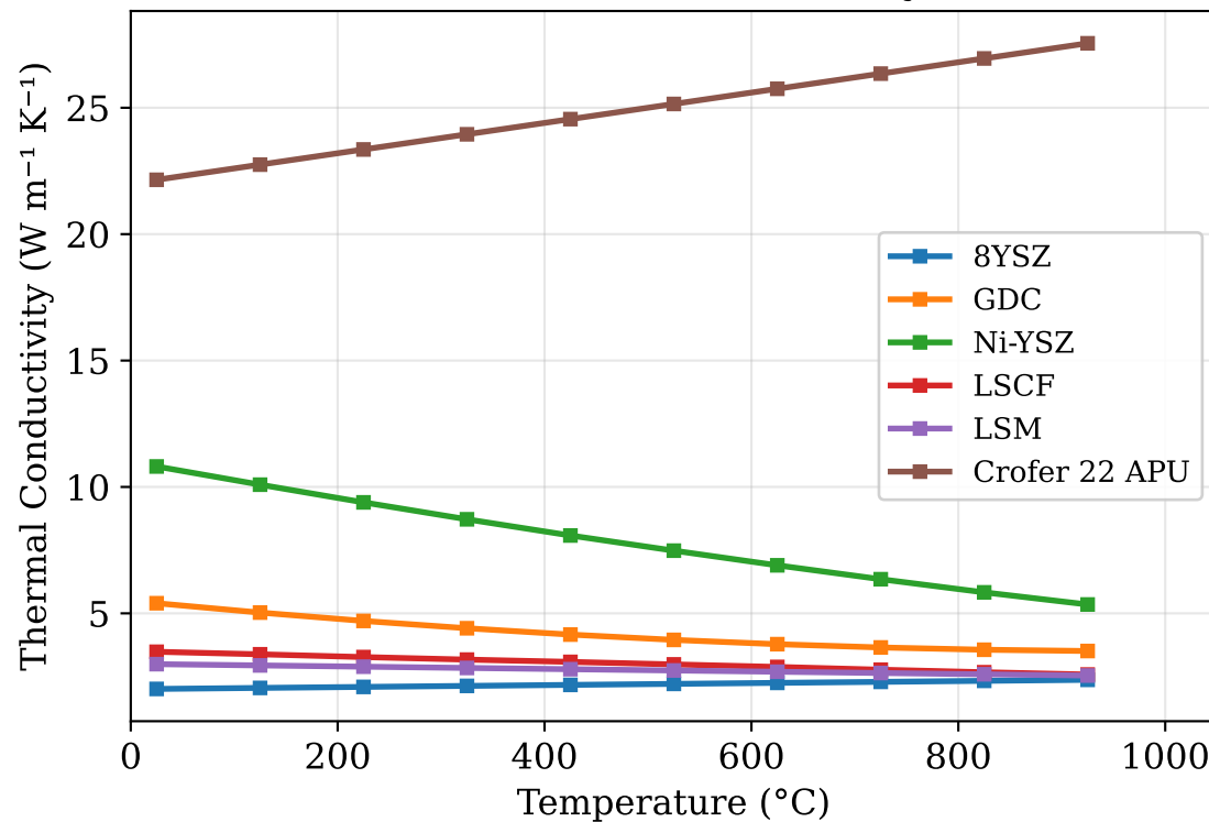
(b) Thermal Conductivity
