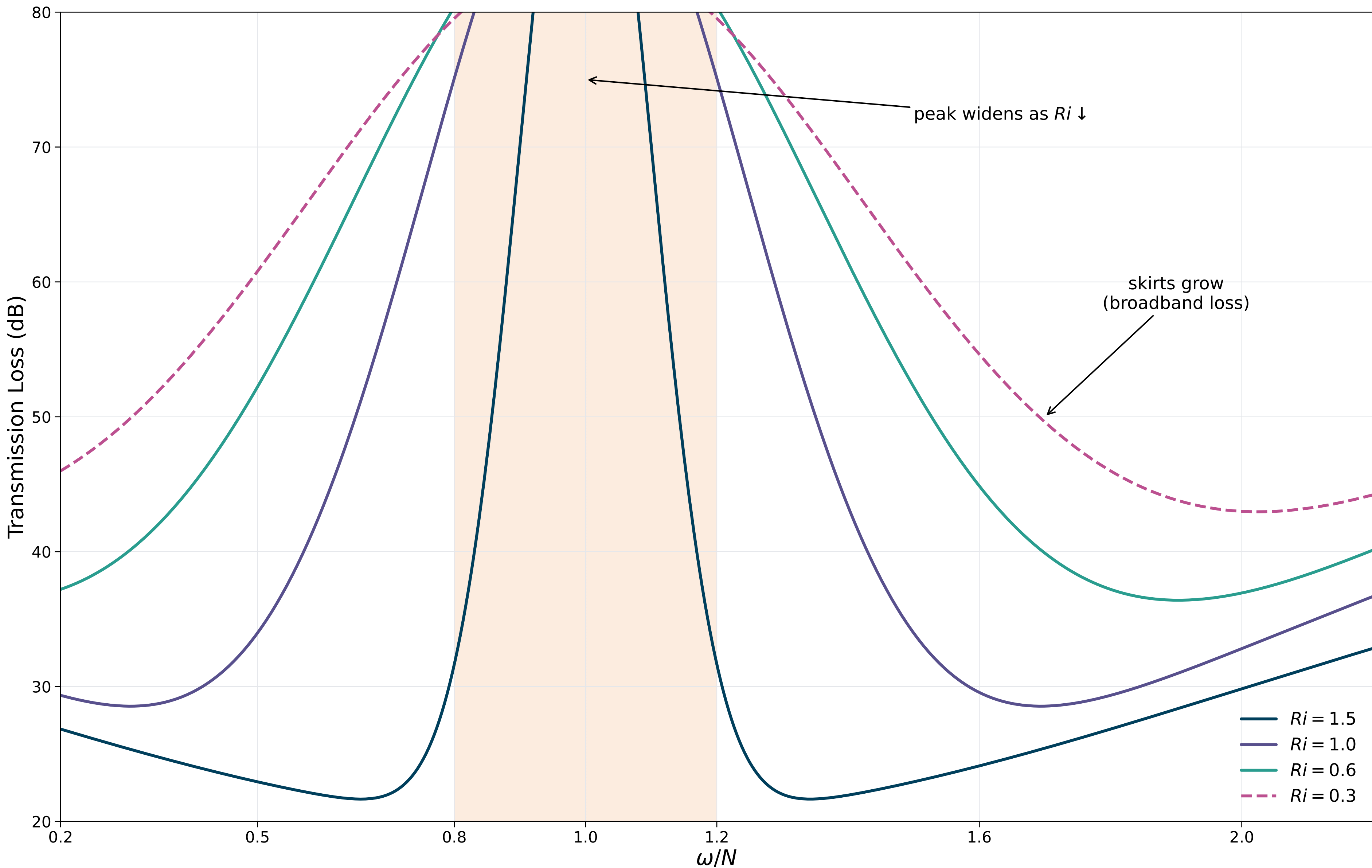
Figure 3.8C — Attenuation vs Frequency
