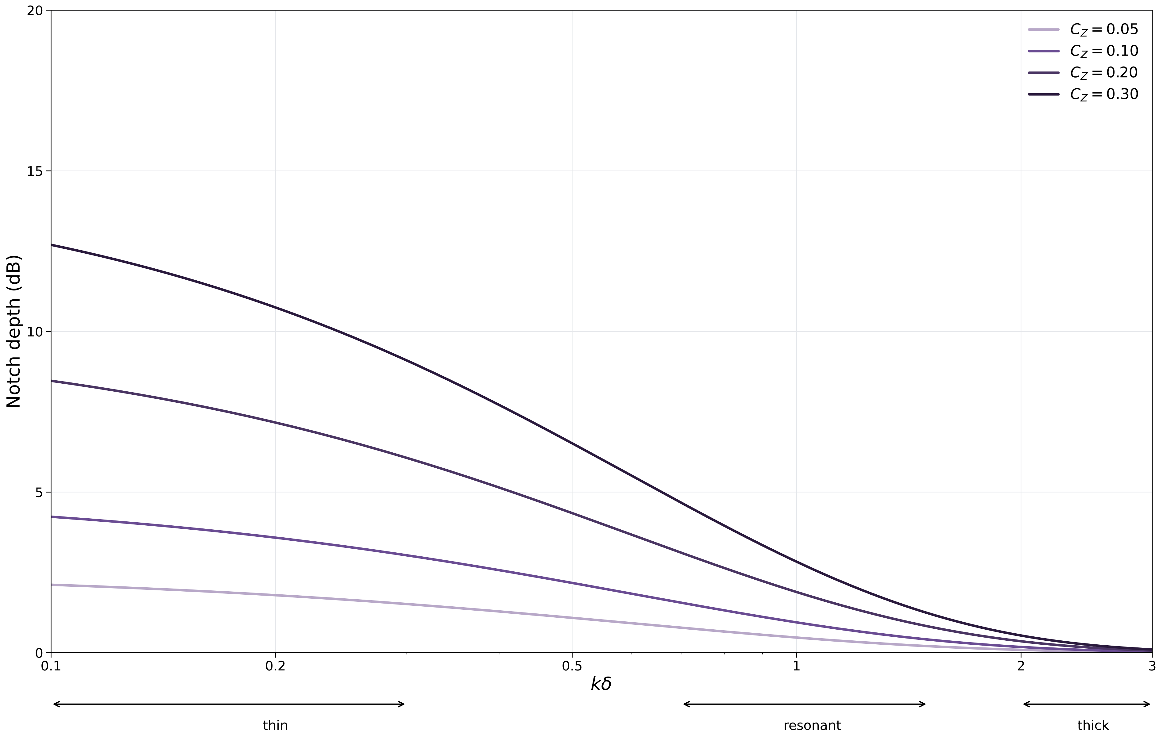
Figure 3.8D — Notch Depth vs Interface Thickness
