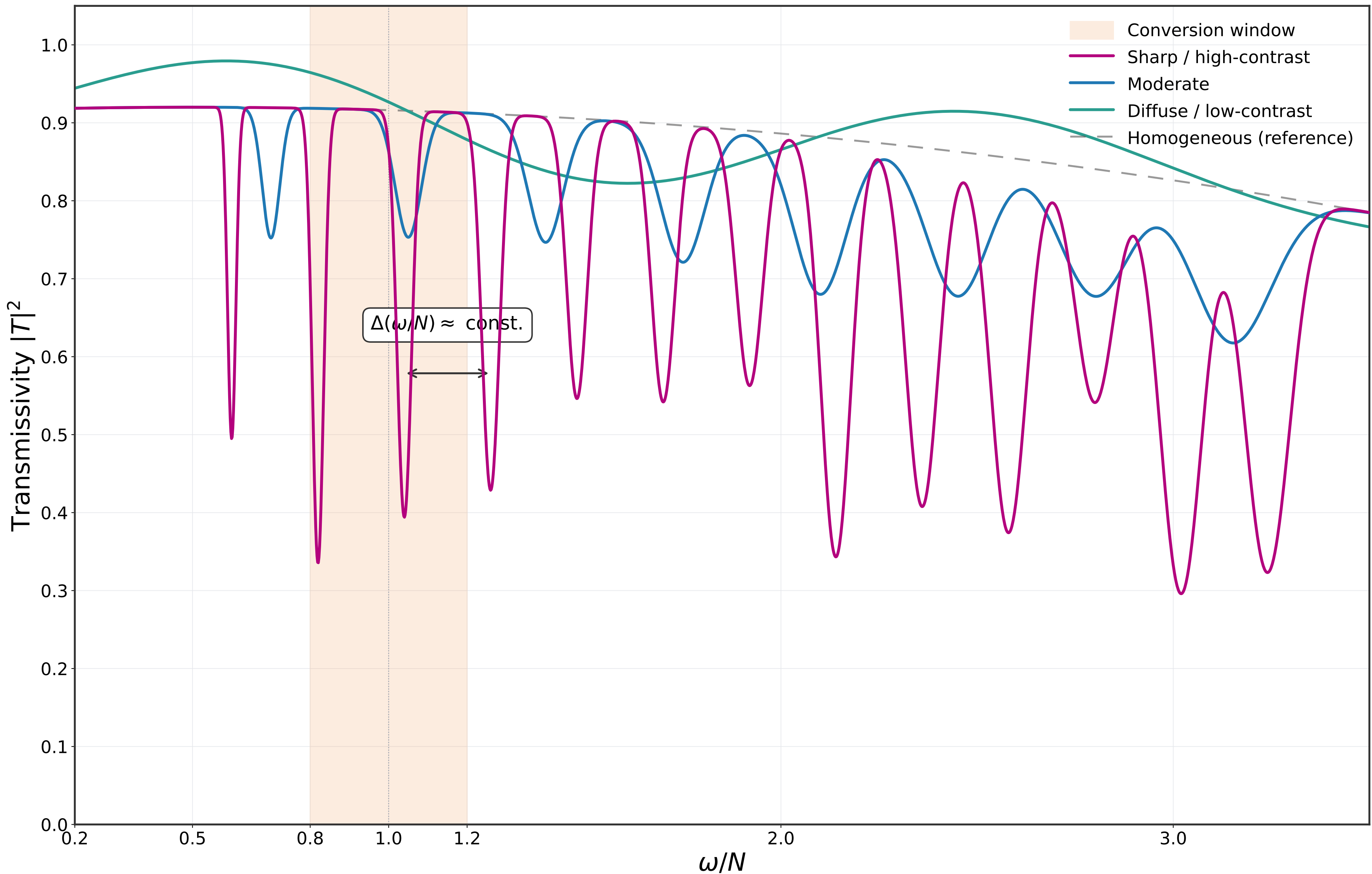
Figure 3.5B. Transmissivity vs normalized frequency across interface regimes. Sharp, high-contrast layers exhibit deep, frequent notches; moderate layers show gentler quasi-periodic structure; diffuse/low-contrast layers are nearly smooth.
