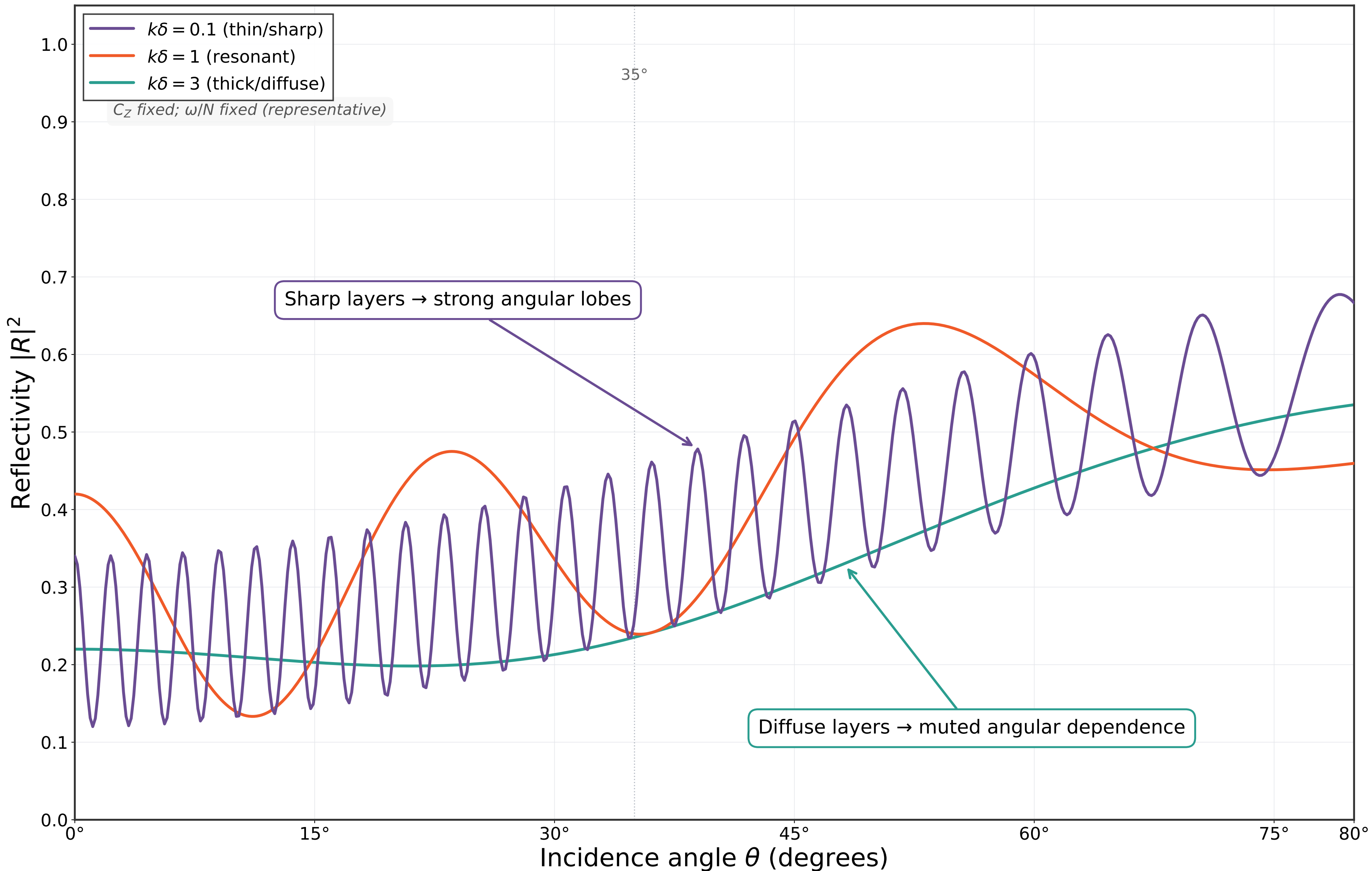
Figure 3.5C. Reflectivity vs incidence for thickness parameter k\delta at fixed contrast. Thin/sharp layers yield pronounced obliquity-dependent lobes; diffuse layers produce smoother, muted trends.
