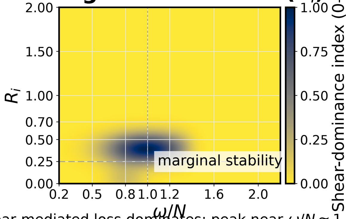
Figure 3.6A — \text{SDI}(R_i, \omega/N)
