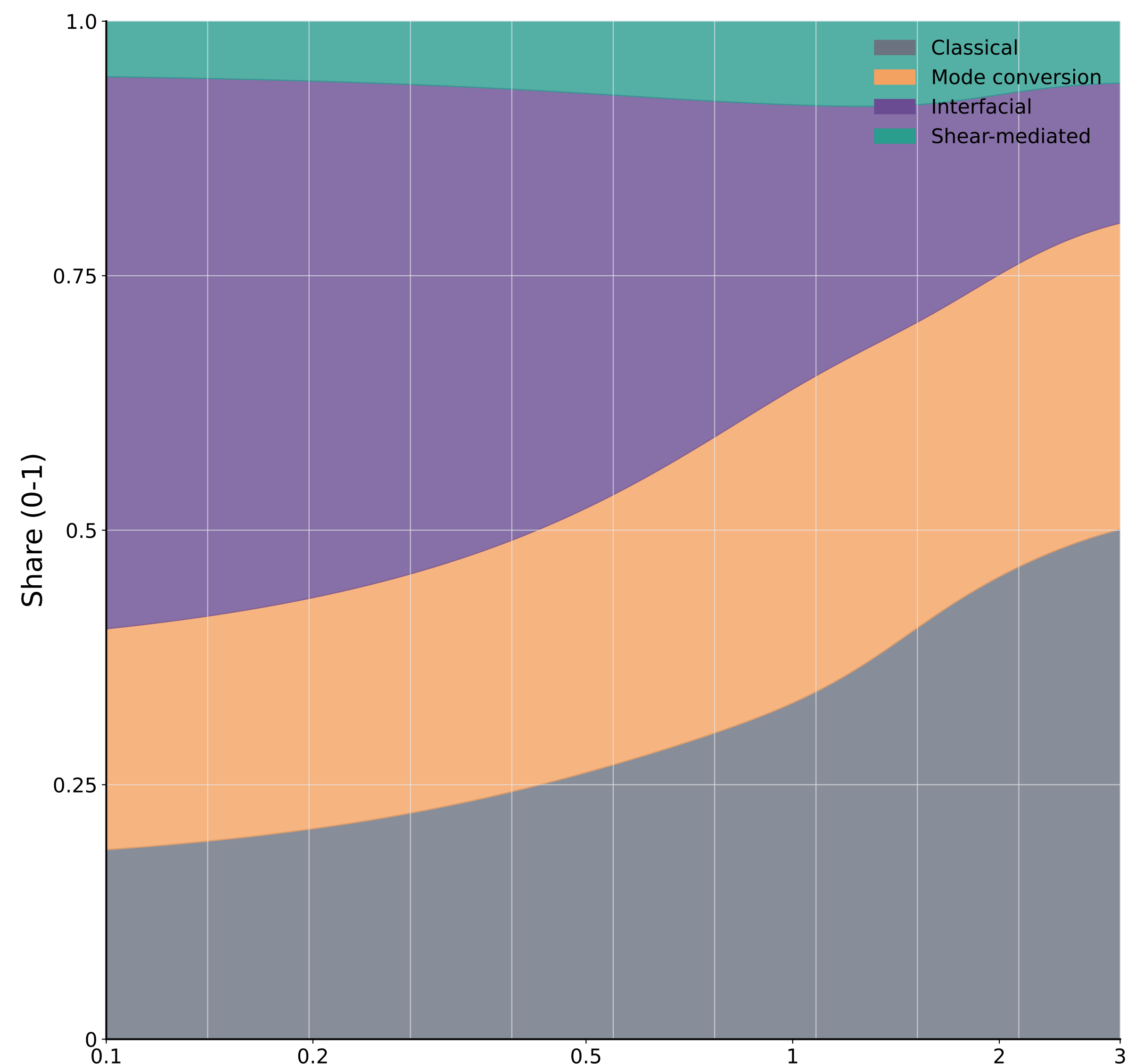
Figure 3.7C1. Interfacial share peaks for sharp, high-contrast transitions (low k\delta ) and decays as the interface becomes diffuse (large k\delta ). Classical share increases complementarily; conversion and shear change little at fixed \omega/N .
