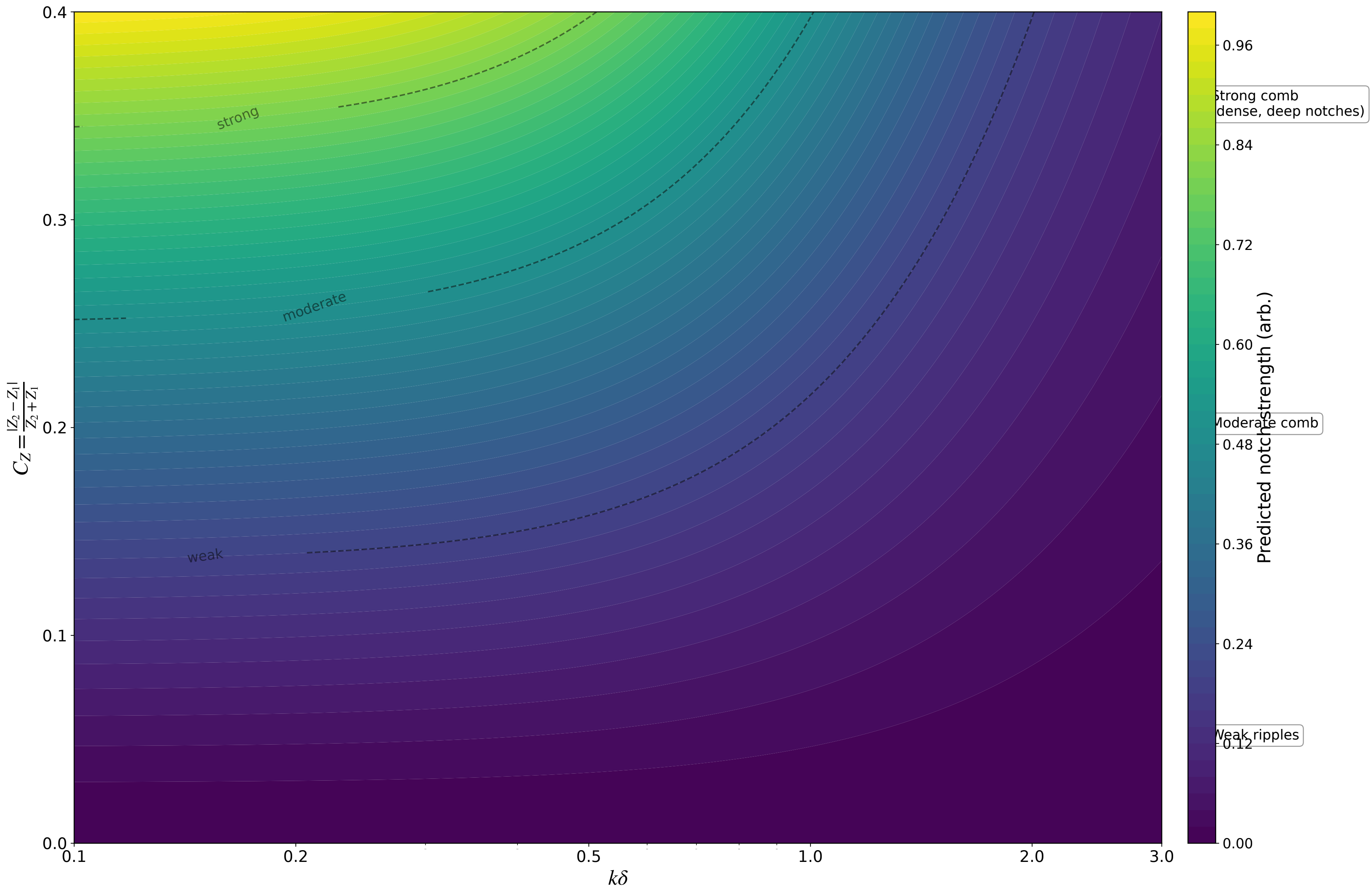
Figure 3.8B. Notch strength increases with impedance contrast C_Z and decreases with interface thickness k\delta ; sharp, high-contrast layers produce strong comb-like reverberation.
