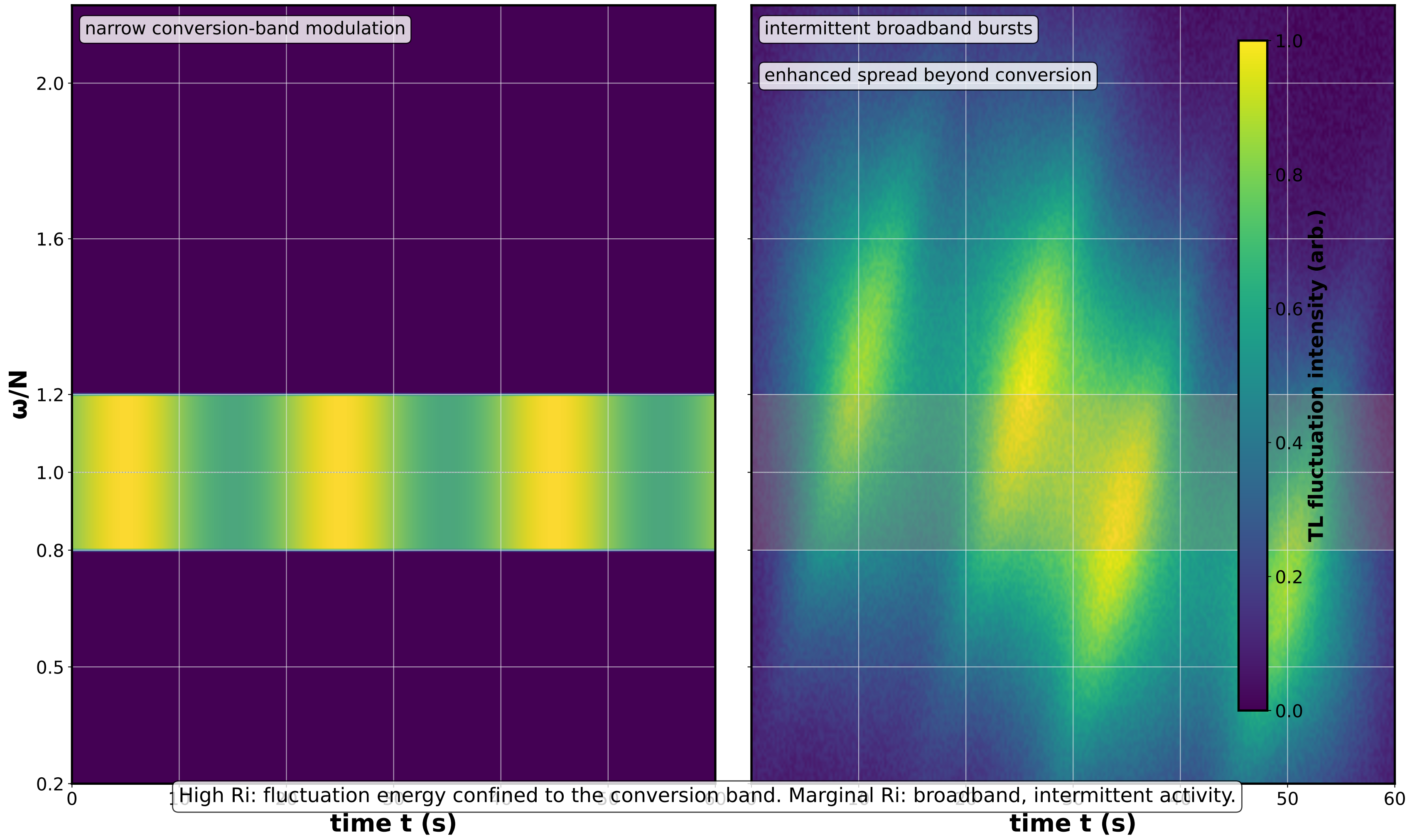
Figure 3.6B — Time-frequency TL fluctuation intensity
