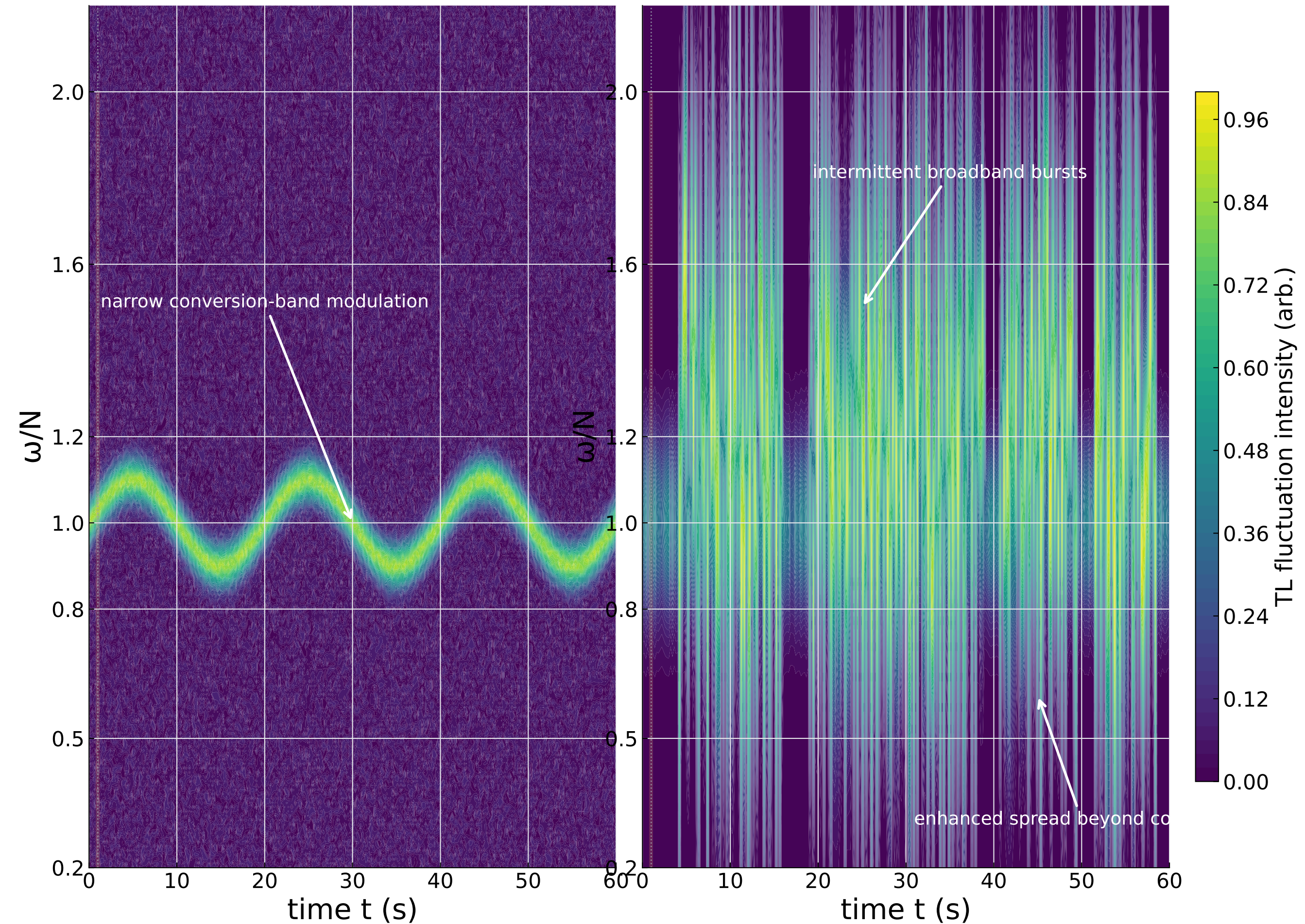
Figure 3.6B — Time-frequency TL fluctuation intensity High Ri Marginal Ri
