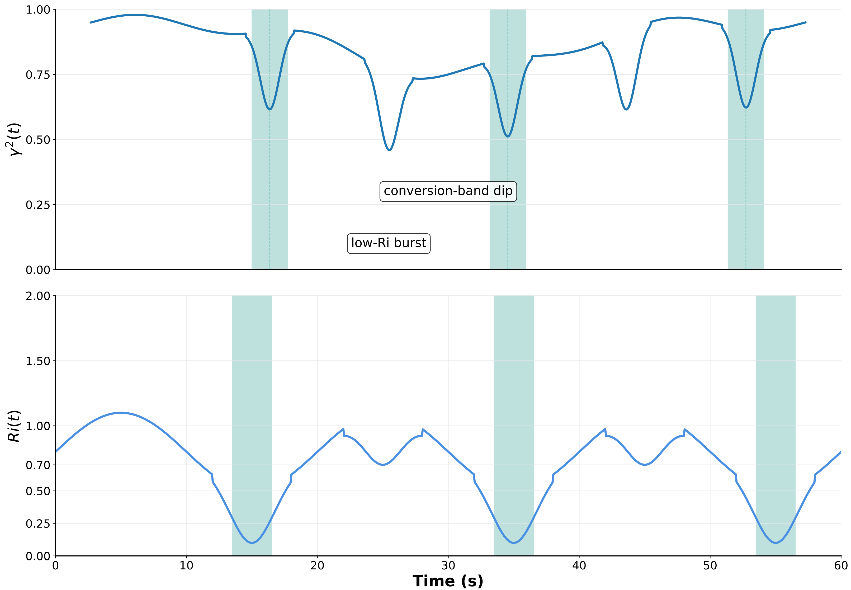
Figure 3.9C. Time correlation between array coherence and Ri(t) : a persistent conversion-band dip plus intermittent losses coincident with low-Ri bursts.
