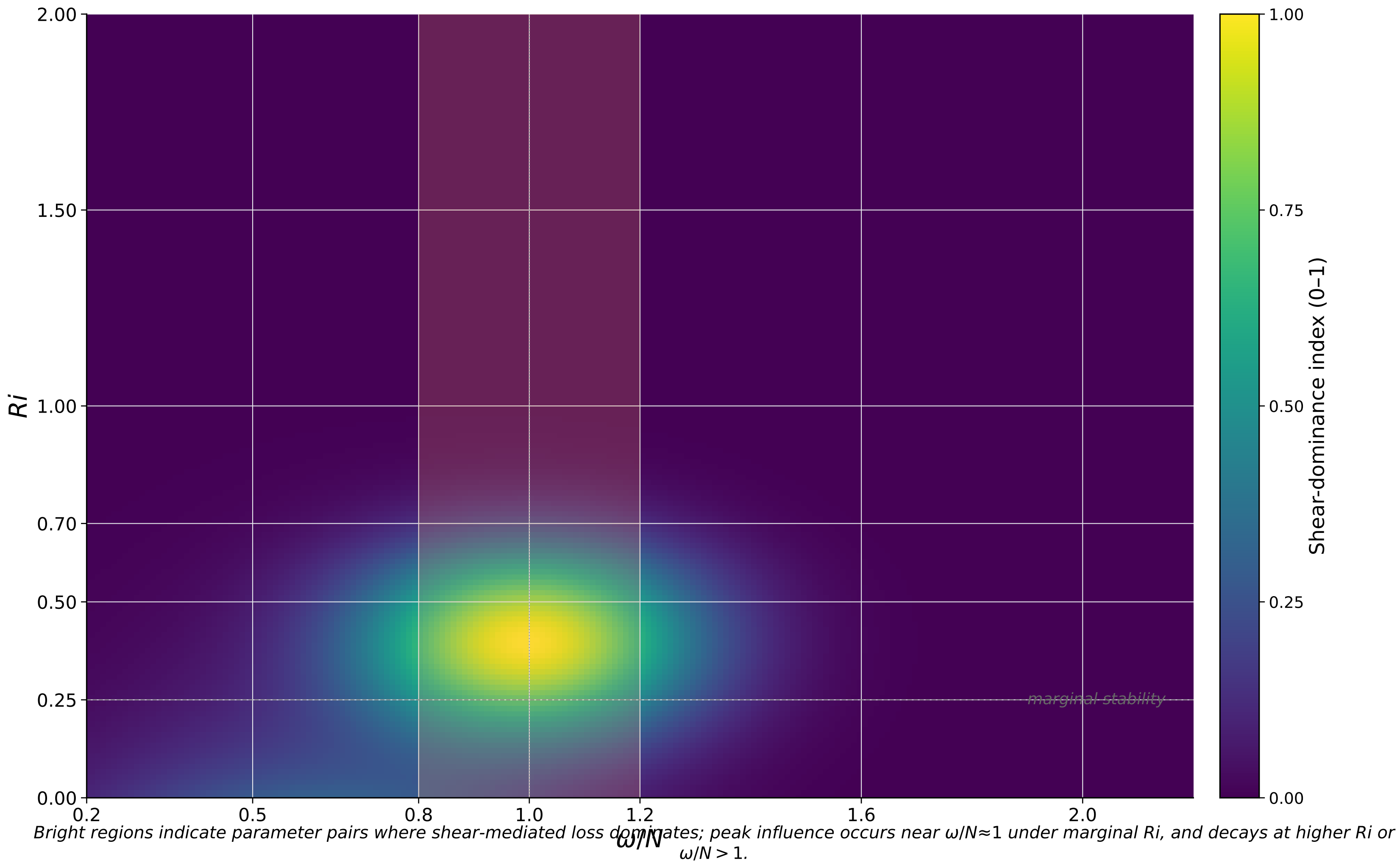
Figure 3.6A — Shear-dominance index SDI(Ri, \omega/N)
