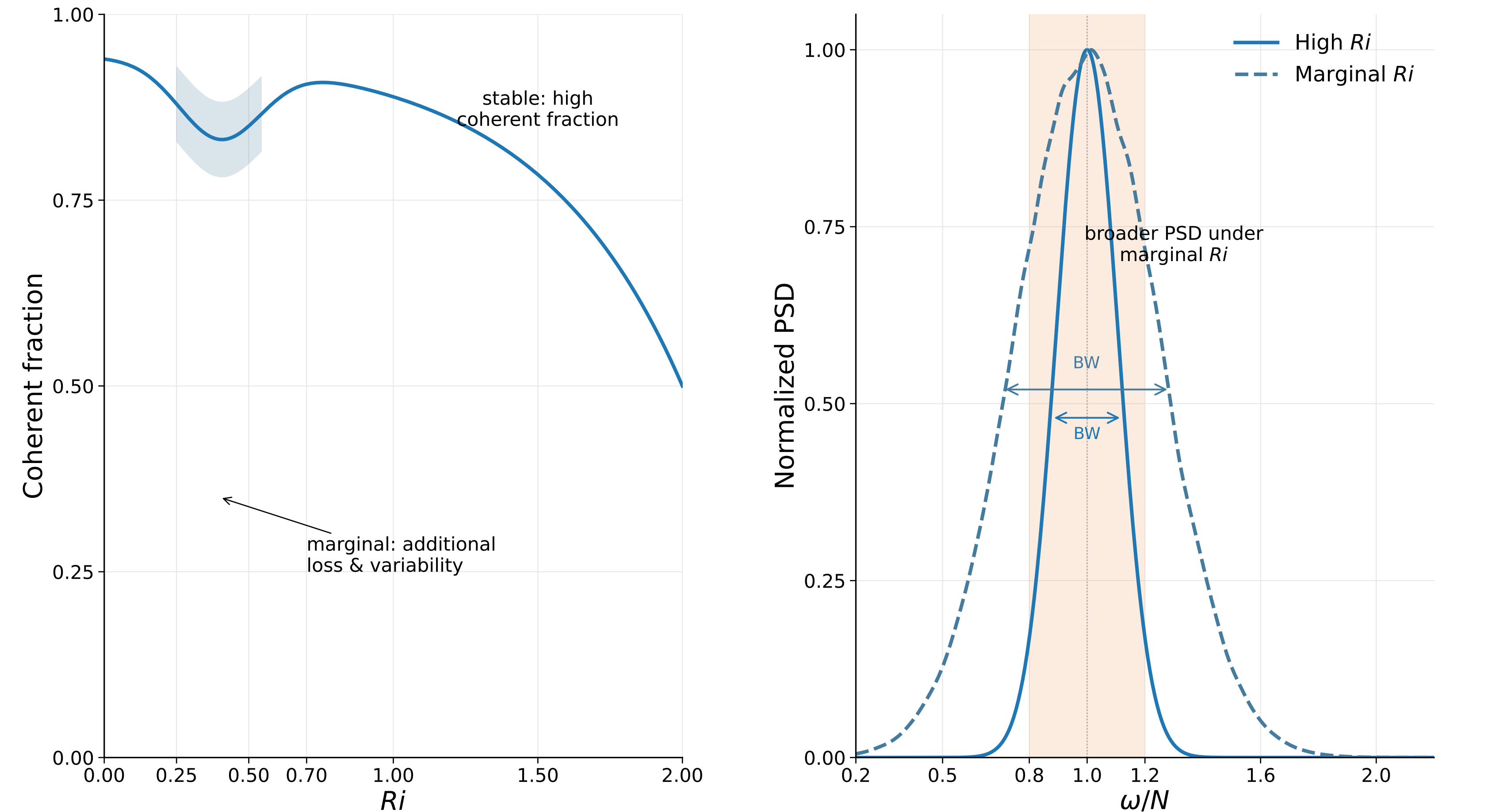
Figure 3.6C — Coherence loss and spectral broadening with decreasing Ri
