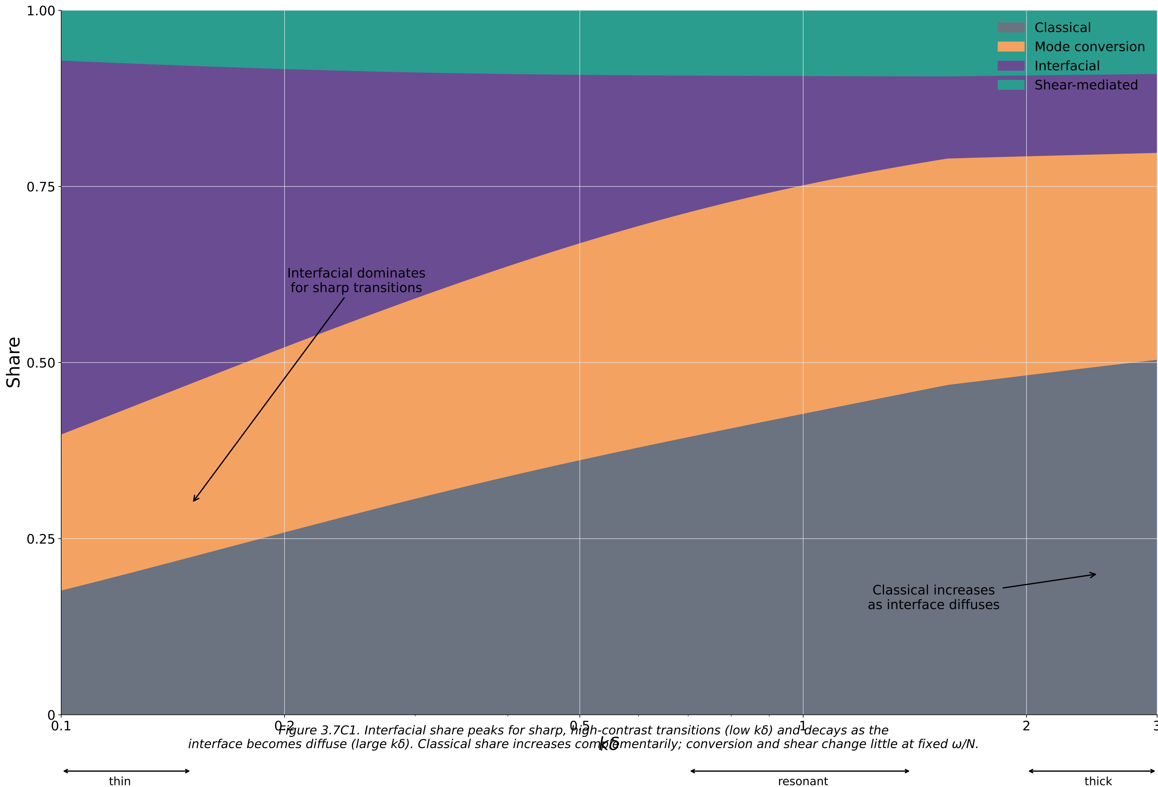
Figure 3.7C1 — Mechanism shares vs k\delta (interface sharpness), fixed \omega/N = 1
