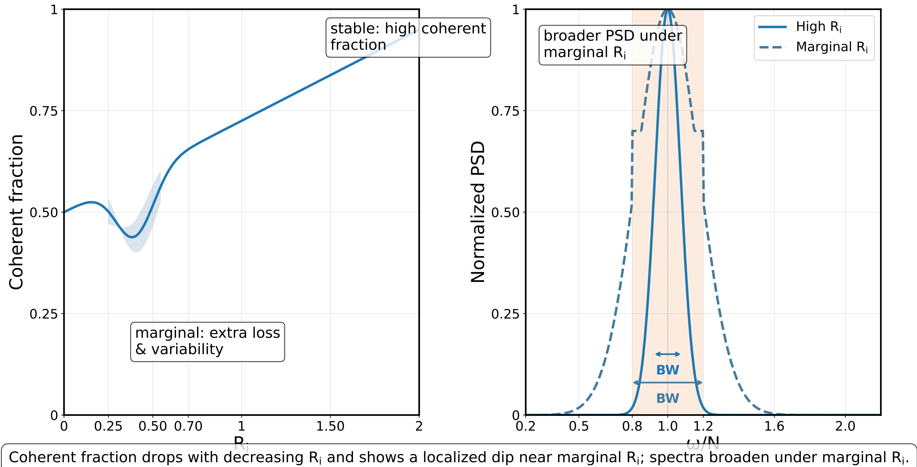
Figure 3.6C — Coherence loss and spectral broadening with decreasing R_i
