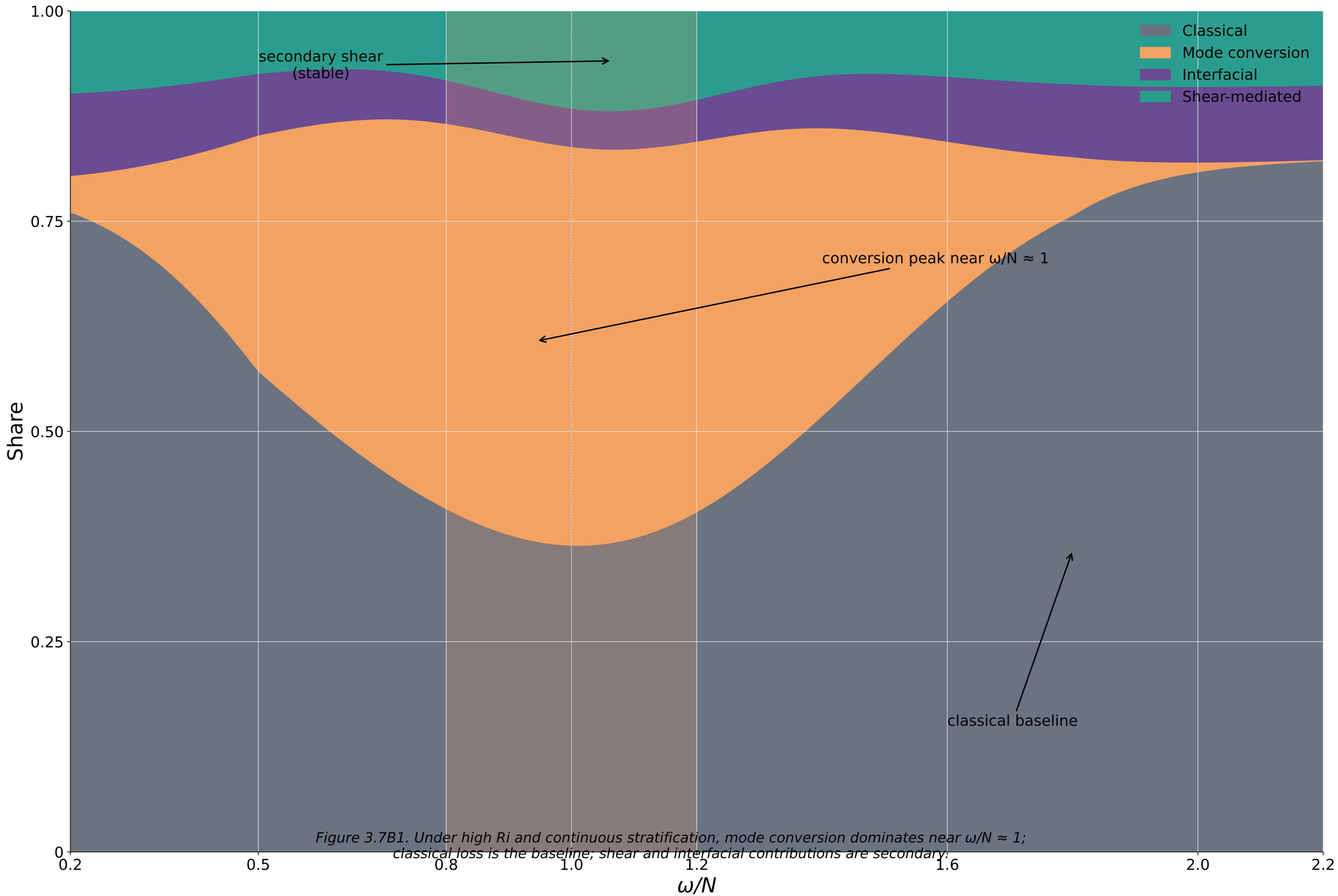
Figure 3.7B1 — Mechanism shares vs \omega/N (High Ri, continuous)
