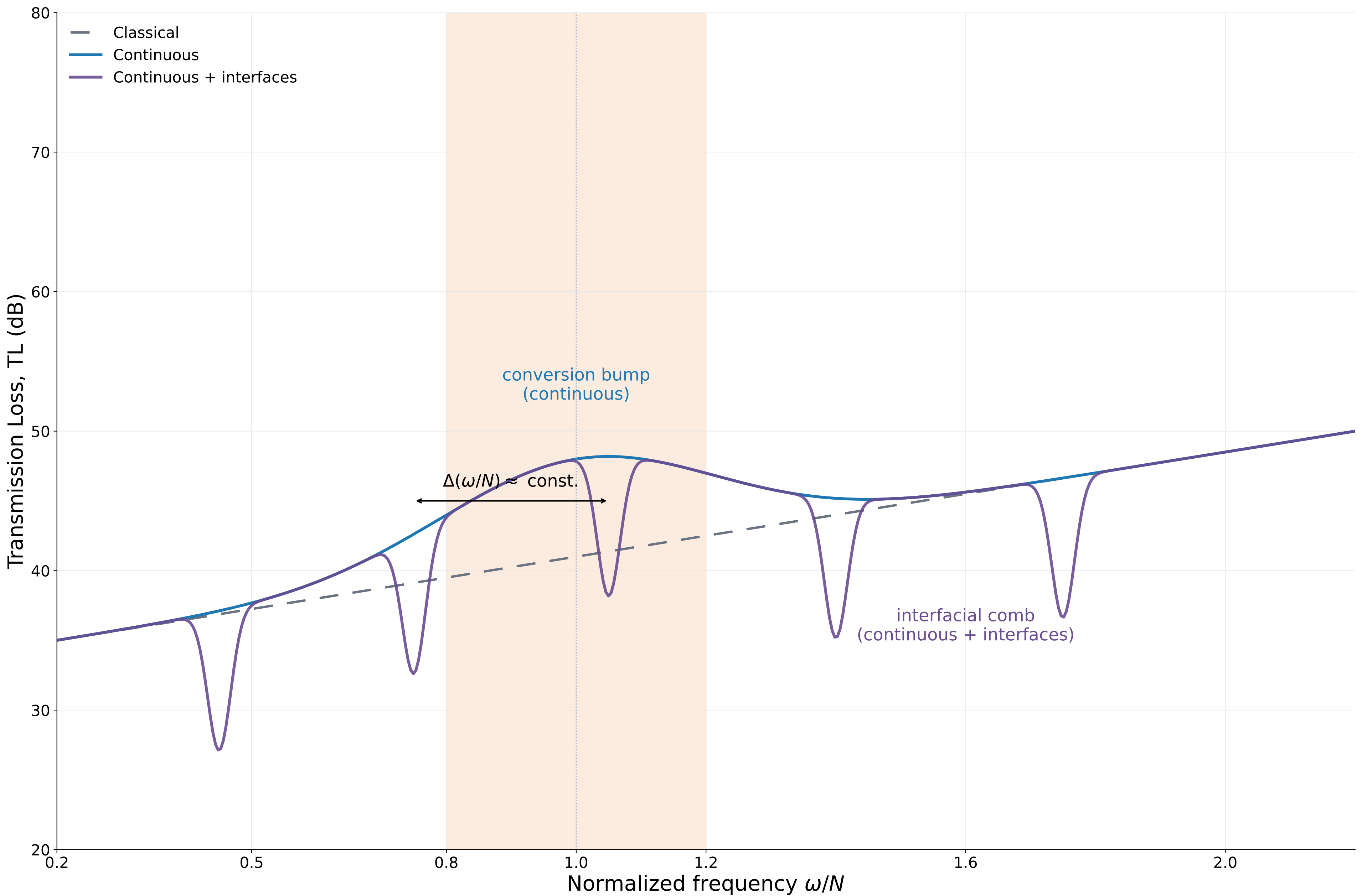
Figure 3.9A. Frequency-sweep signatures: a broad conversion bump at \omega/N \approx 1 for continuous stratification; adding sharp interfaces imposes narrow spectral notches on top of the bump.
