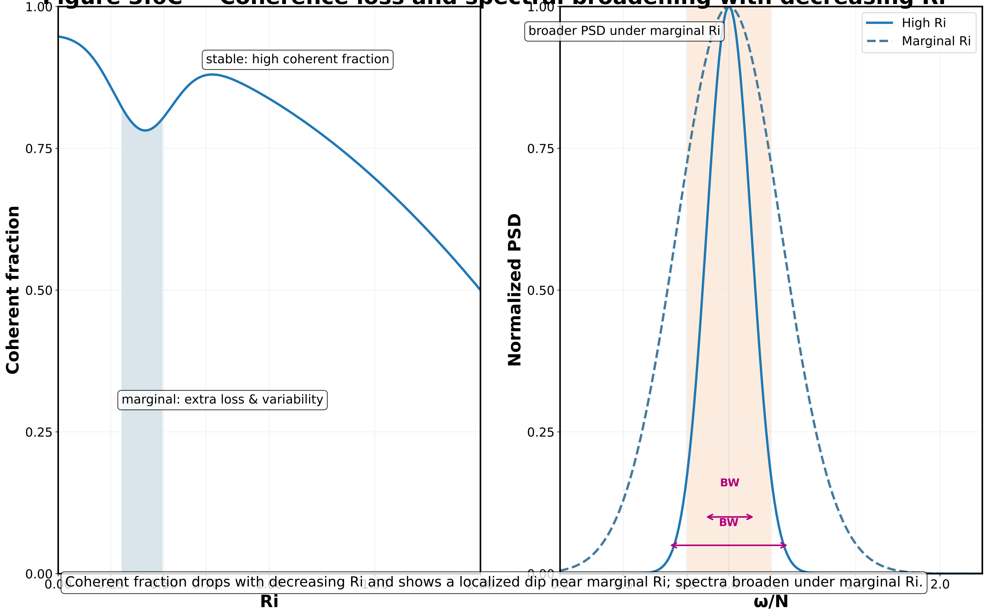
Figure 3.6C — Coherence loss and spectral broadening with decreasing Ri
