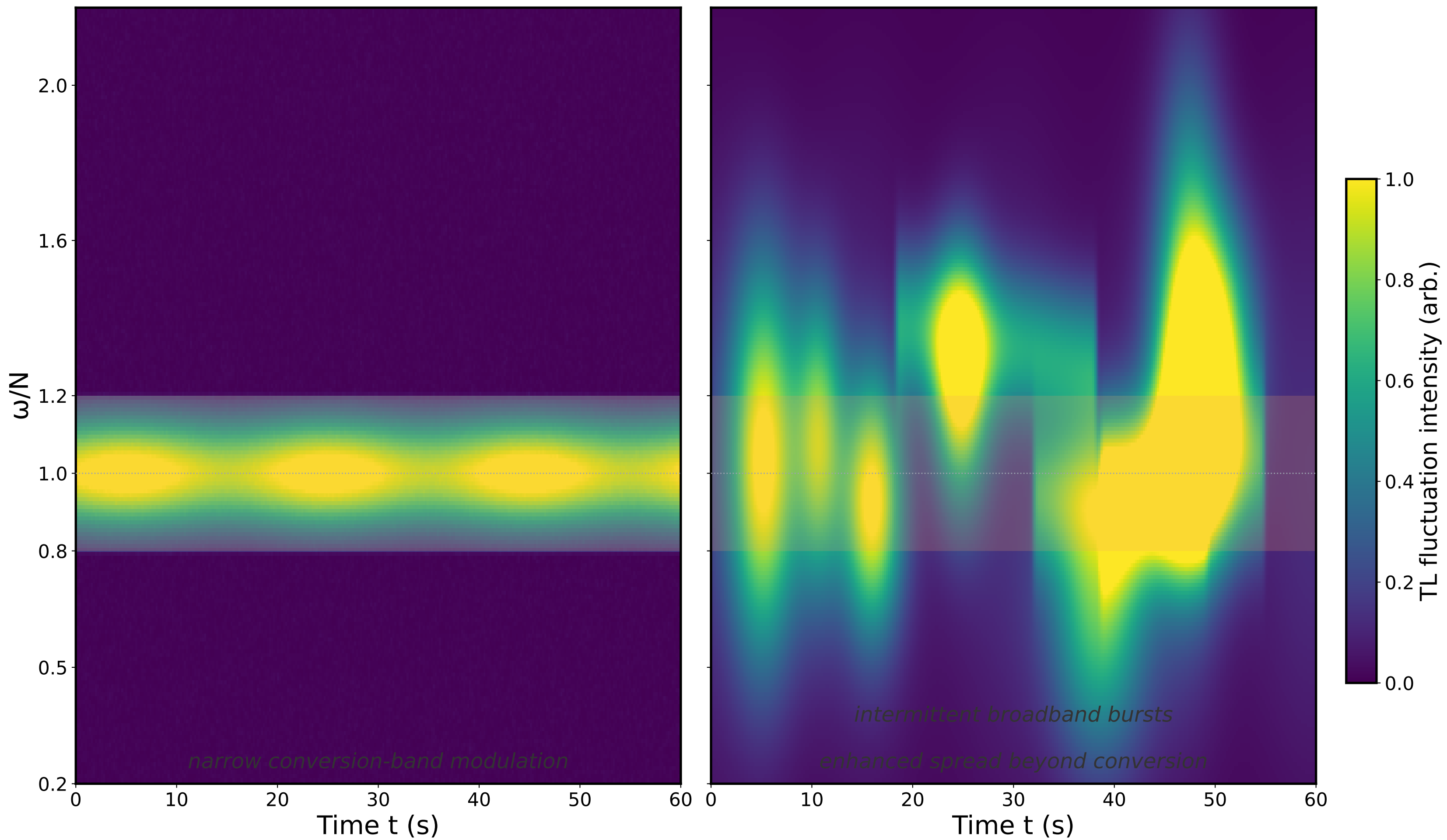
Figure B9.6B — Time-frequency TL fluctuation intensity
