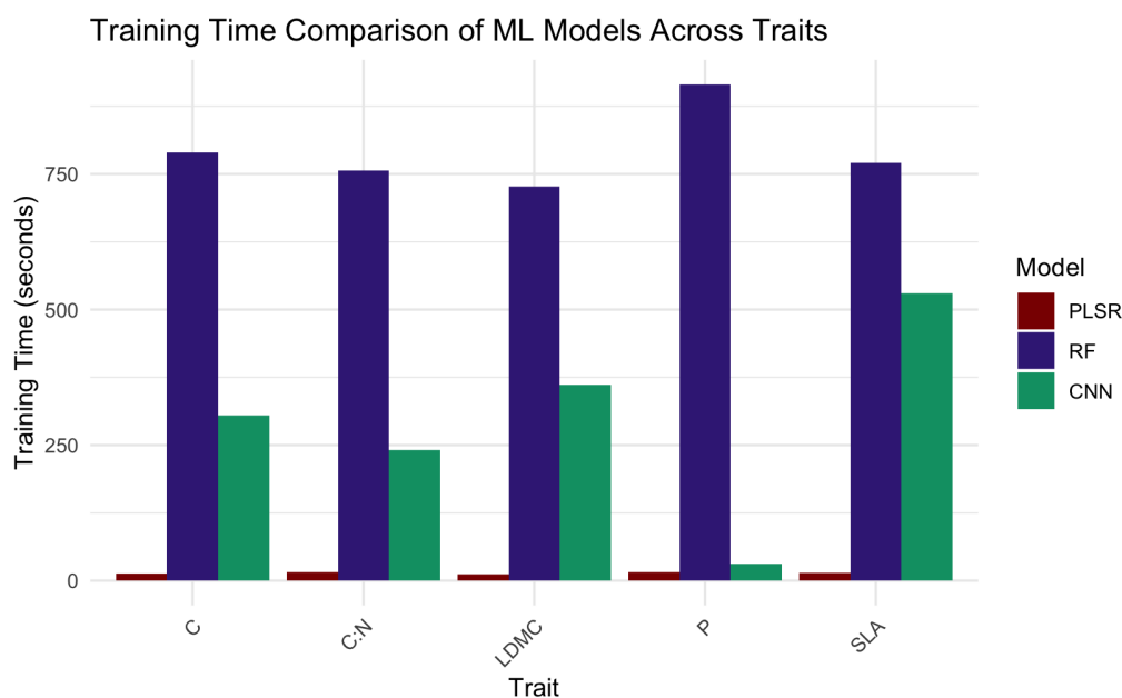
Figure 4.4: This visualizes the training time (in seconds) required for different machine learning models (PLSR, RF, CNN) across various plant traits.
