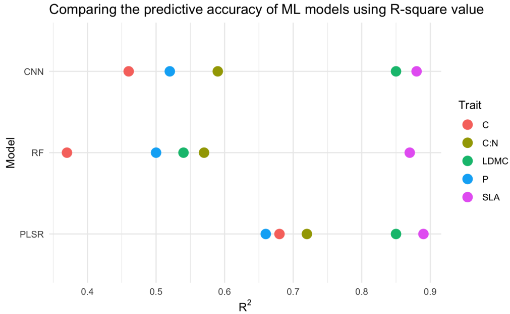
Figure 4.1: Scatter plot comparing the R^2 values of different traits across three ML models
