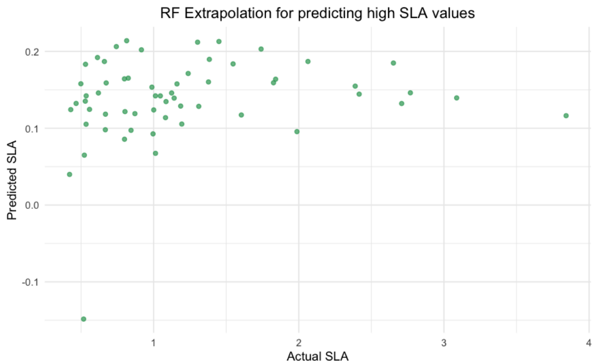
Figure 3.22: The scatter plot illustrates the predicted versus actual SLA values for the extrapolation of the random forest model on the upper data range
