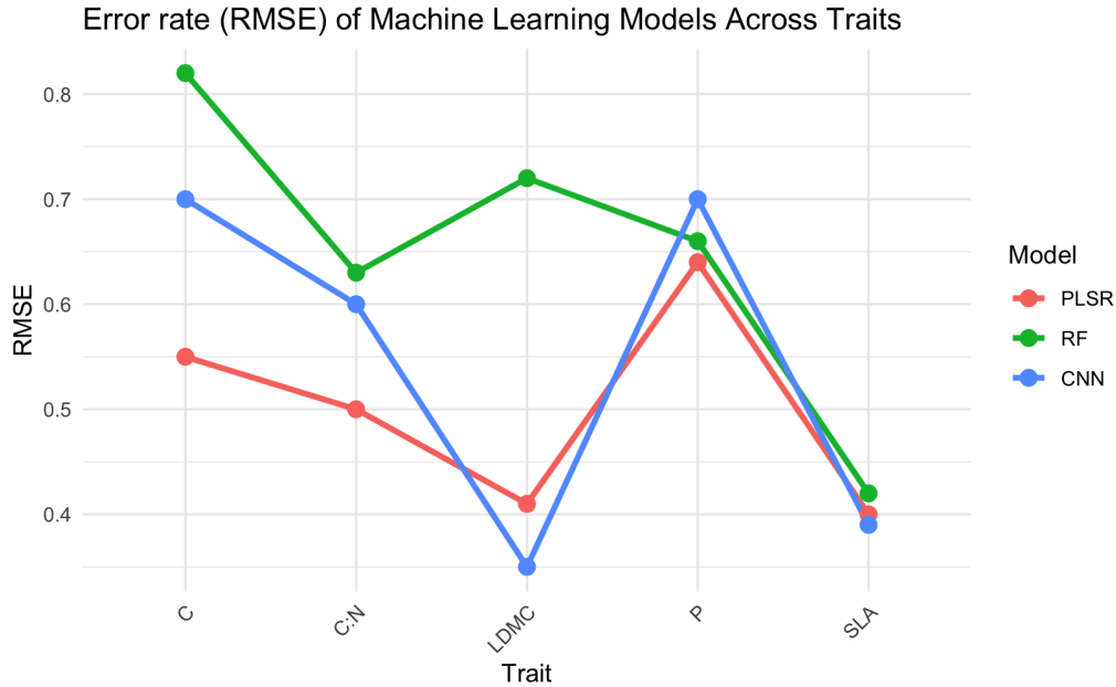
Figure 4.2: Distribution of RMSE values across all ML models in leaf trait analysis.
