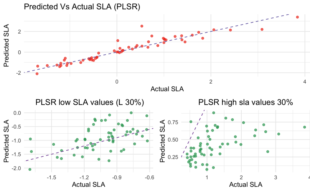
Figure 4.6: This scatter plot presents the extrapolation results as well as the normal PLSR prediction o the SLA trait. It shows the difference in predictive accuracy when tested on higher and lower data ranges.
