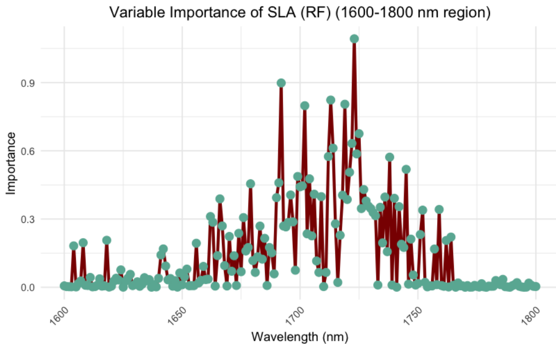
Figure 4.10: Zoomed-in view of variable importance of SLA in RF within the 1600 to 1800 nm range (Figure 4.9)
