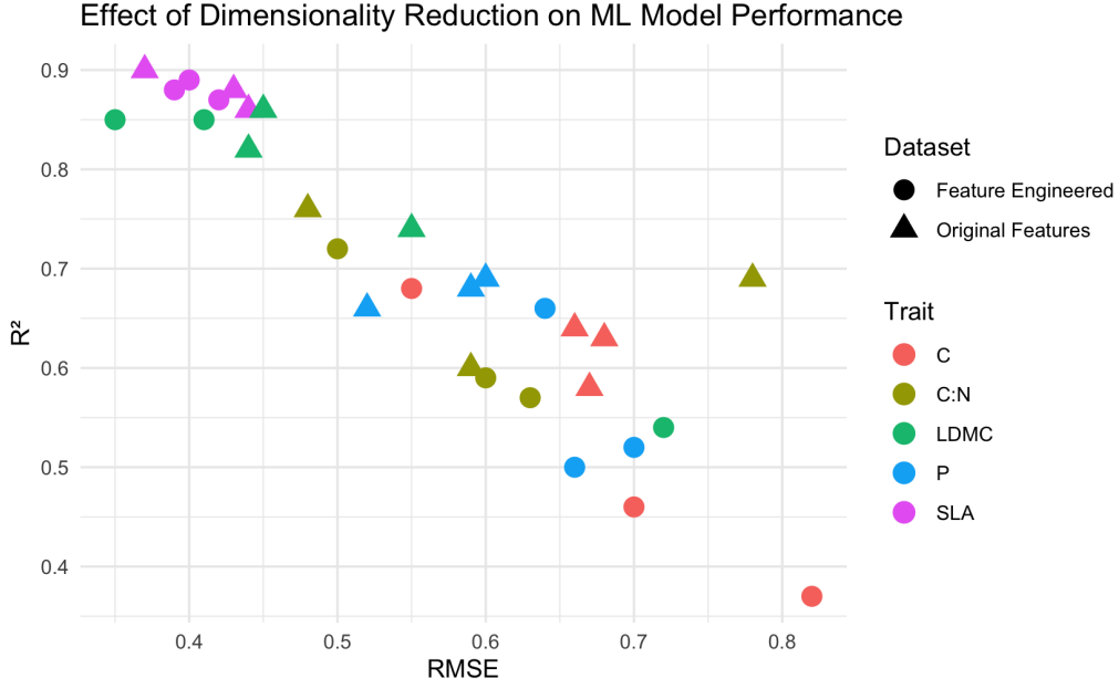
Figure 4.11: This plot illustrates the effect of dimensionality reduction in all three ML models across all traits.
