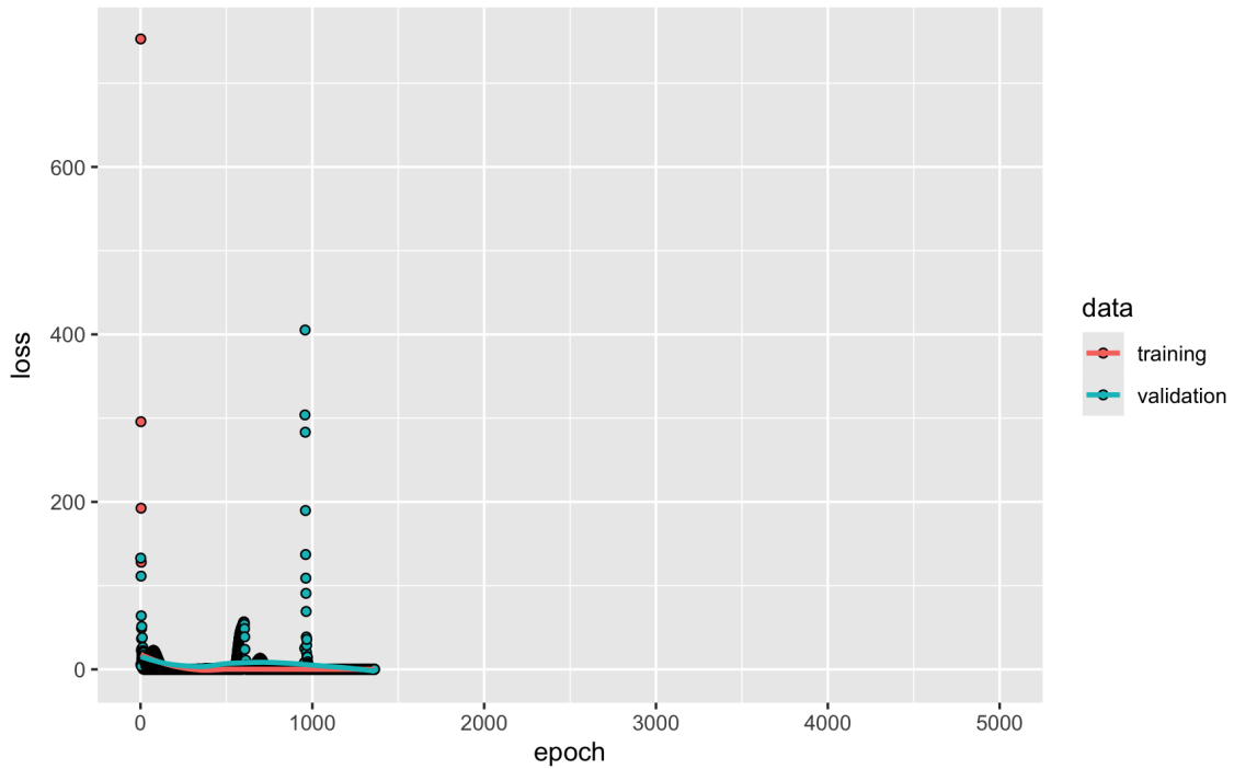
Figure 4.5: The CNN training model for SLA trait, illustrating the training and validation loss during training the model. The original model’s training was set to 5000 epochs, and it stopped before reaching 1500 epochs.
