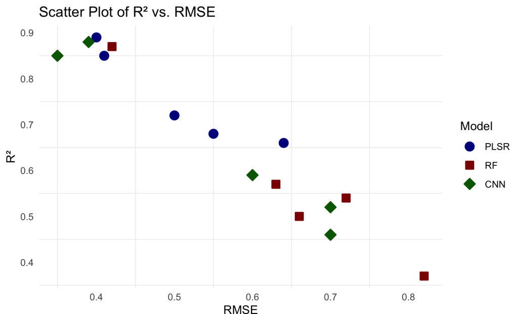
Figure 4.3: Scatter plot comparing the R^2 and RMSE of all three ML models
