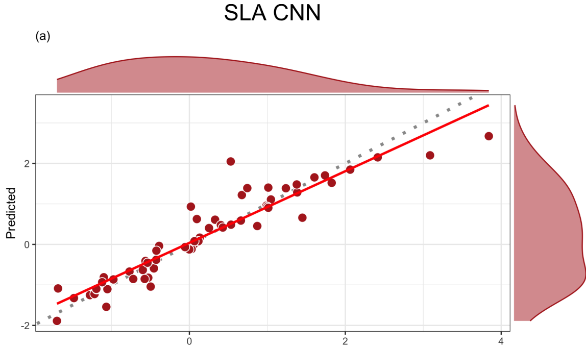
Figure 3.20: This plot illustrates the predictive ability of CNN for SLA trait. The dotted line represents perfect prediction and the red line represents relationship between predicted and measured values based on the linear regression. The closer the red and dotted lines are, the better the prediction. The colored regions in the margins represents distribution of the predicted and measured values.
