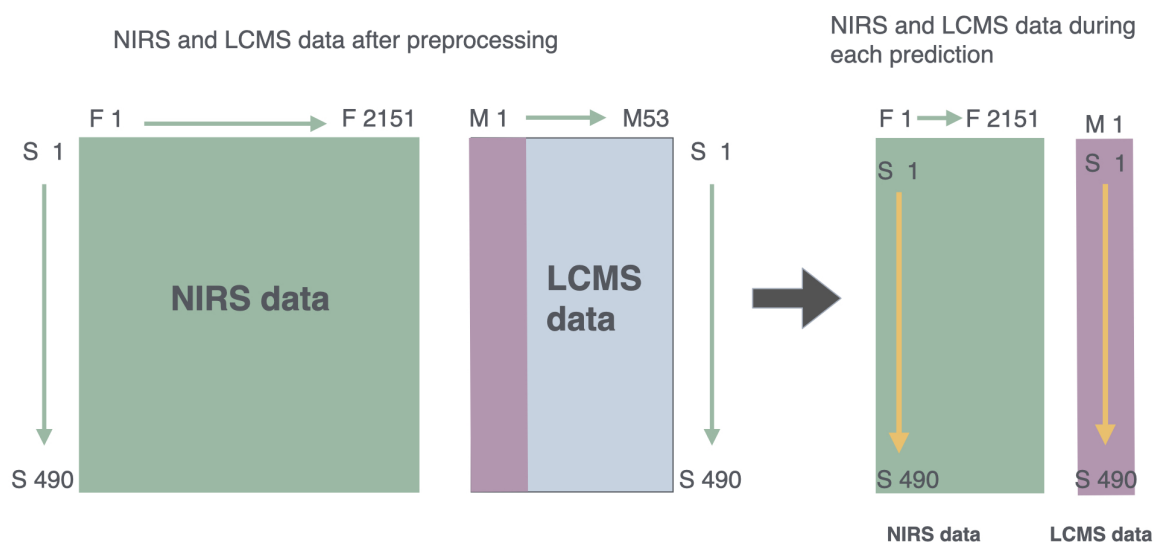
Figure 3.23: Schematic representation of the prediction of LCMS features from NIRS data with "F" representing features, "S" stands for samples and "M" for metabolites. During each iterations, a single metabolite column is selected (vector) and is then predicted using NIRS data matrix with each sample row of NIRS data(sample spectra) predicting the LCMS data corresponding to that sample.
