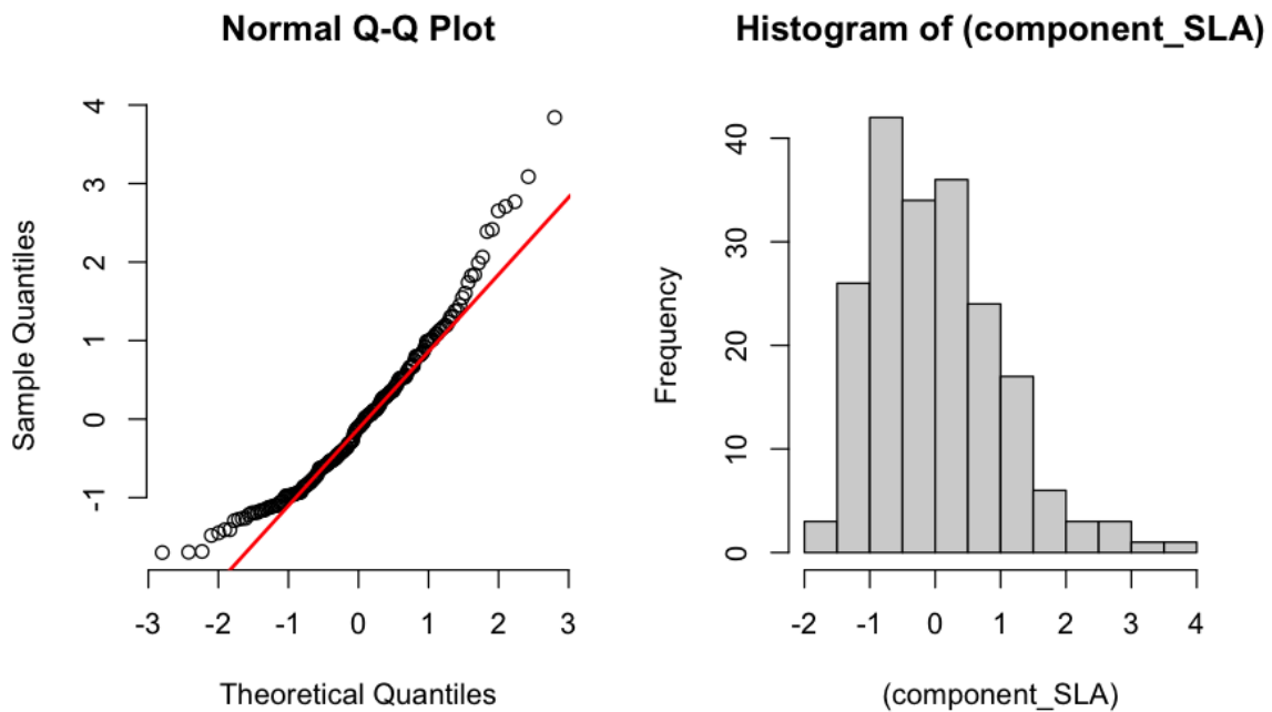
Figure 3.18: Q-Q plot (left) illustrating normality of SLA and histogram (right) showing the distribution of SLA (scaled version) values [15]. The Q-Q plot compares the quantiles of component SLA (Y axis) to the quantile of normal distribution (X axis). Data points closer to the redline has the normal distribution. Deviation from this line indicates the presence of outliers. The histogram shows the frequency of distribution of the scaled SLA values. A perfectly normal distribution will result in a bell shaped histogram.
