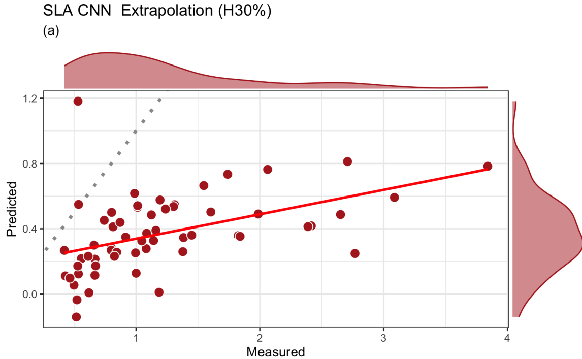
Figure 4.7: The scatter plot illustrates the predicted versus actual SLA values for the extrapolation of the convolutional neural network model on the upper data range. The grey dotted line represents perfect prediction and the red line represents relationship between predicted and measured values based on the linear regression.
