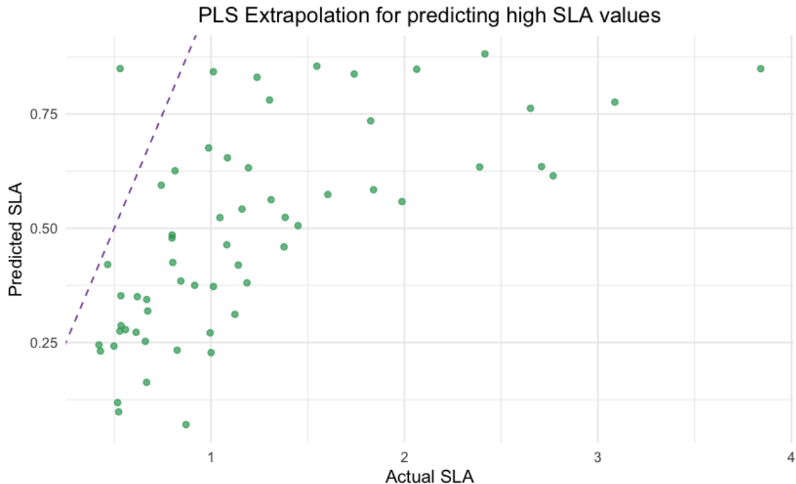
Figure 3.21: The scatter plot illustrates the predicted versus actual SLA values for the extrapolation of the PLSR model on the upper data range.
