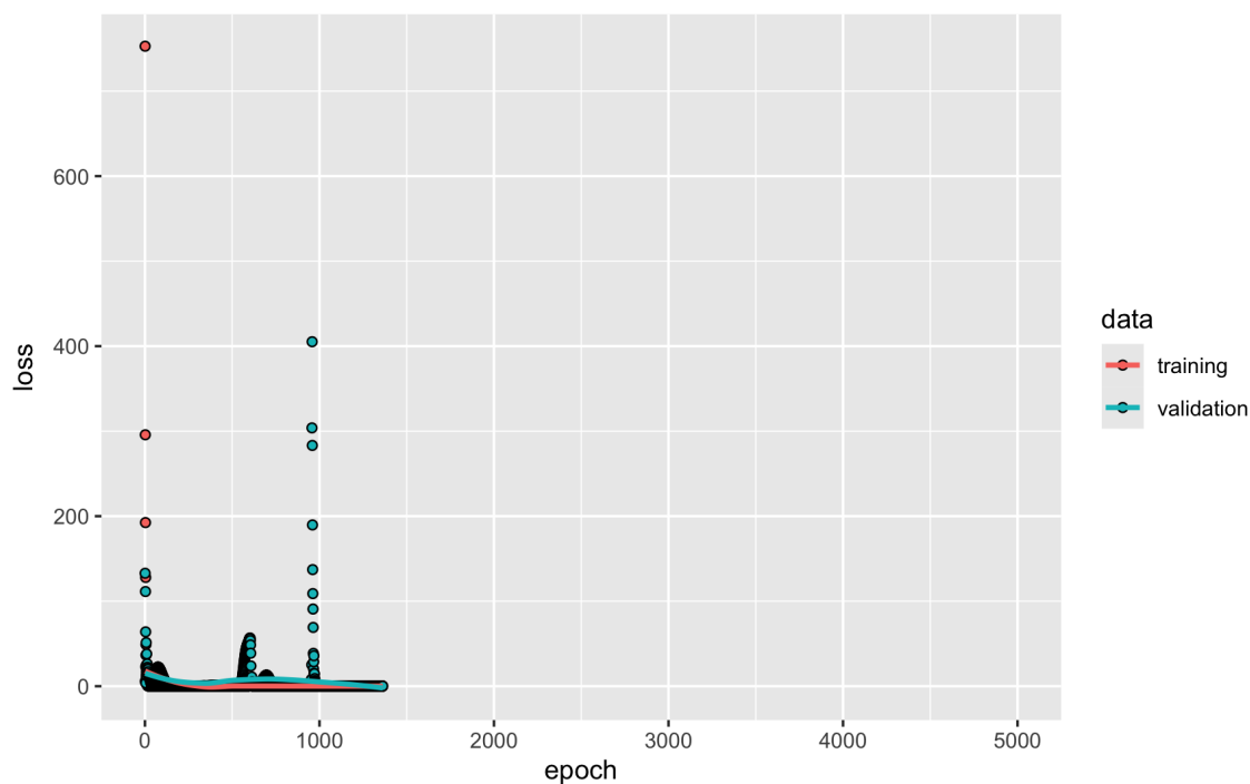
Figure 3.19: The CNN training model for SLA trait, illustrating the training and validation loss during training the model. The model's training was set to 5000 epochs and it stopped before reaching 1500 epochs.
