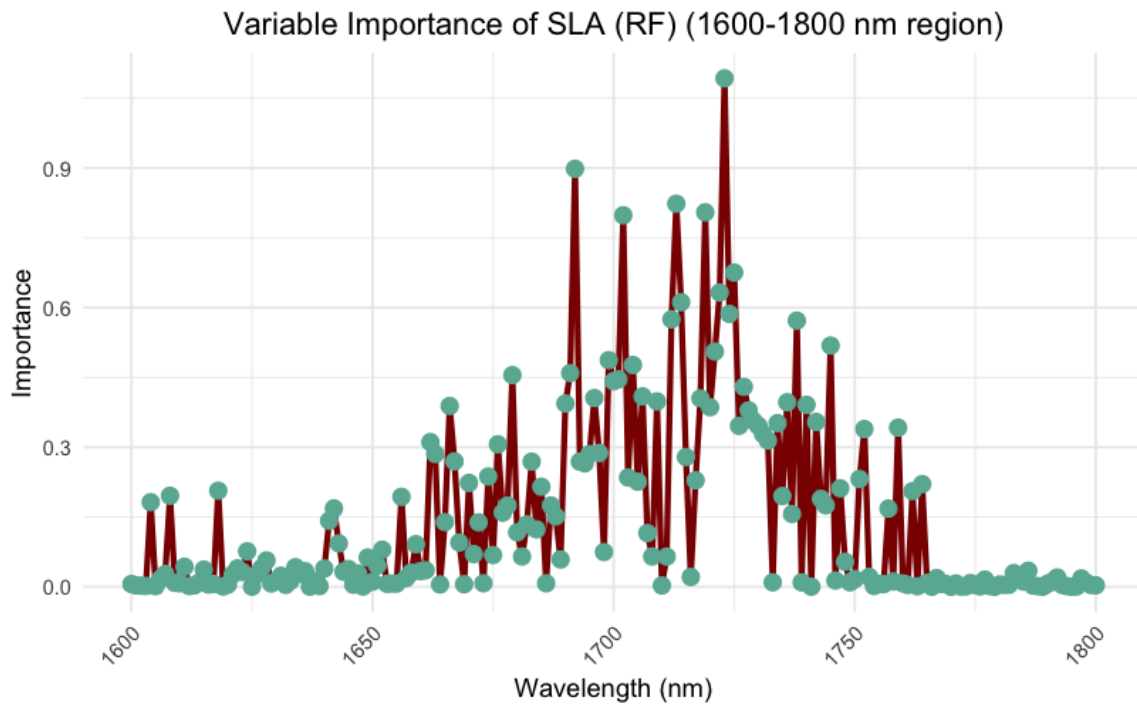
Figure 3.26: Zoomed-in view of variable importance of SLA in RF within the 1600 to 1800 nm range (figure 3.25)
