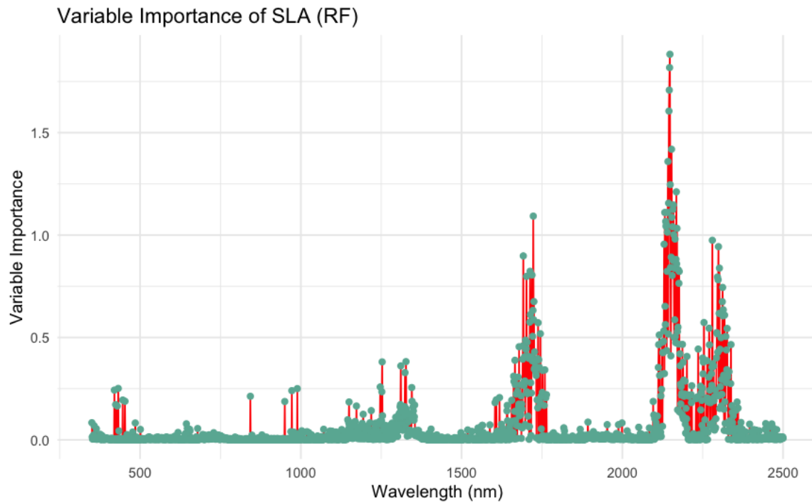
Figure 3.25: Variable importance graph of SLA trait in random forest model
