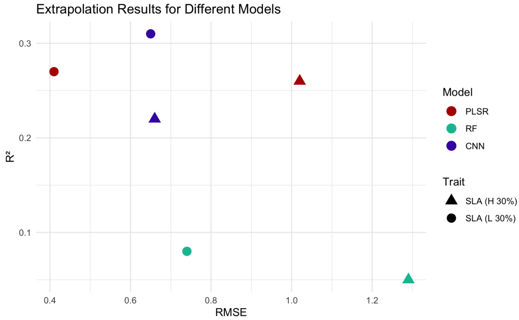
Figure 4.5: Scatter plot presenting the extrapolation results for different machine learning models. The H 30% indicating the model trained with the lower 70% of data and then tested with the highest 30%. The L 30% indicates the model being trained with higher 70% of data and then subjected to testing with the rest of the data.
