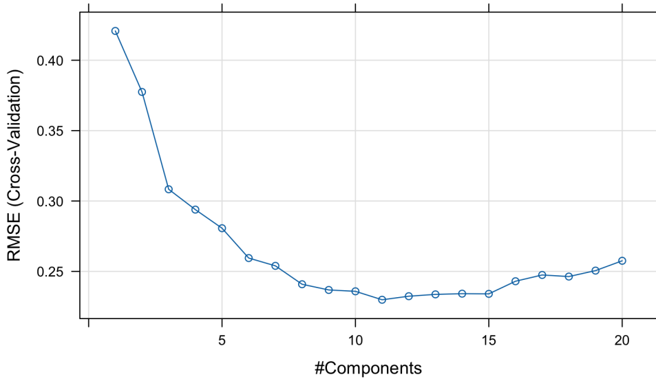
Figure 3.13: Plot of PLSR model for SLA trait prediction illustrating how the number of components were selected. A total of 20 components were considered but only 11 are selected considering different metrics, one being RMSE. This plot shows component 11 has the lowest RMSE value.
