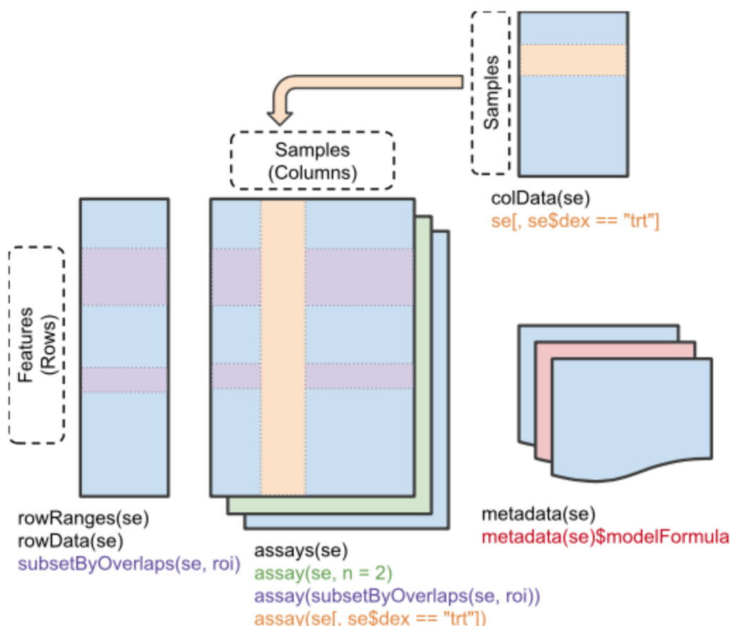
Figure 3.3: Architecture of SummarizedExperiment[55]
