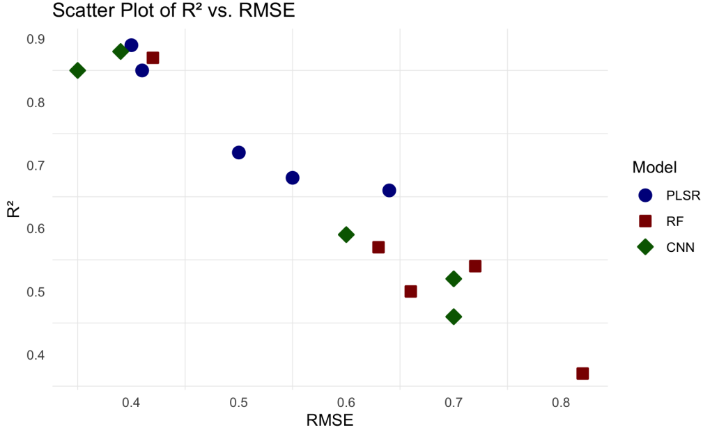
Figure 4.4: Scatter plot comparing the R^2 and RMSE of all three ML models
