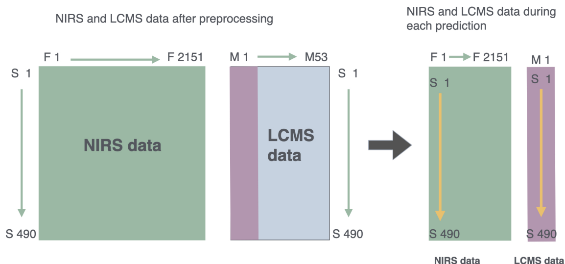
Figure 3.28: Schematic representation of the prediction of LCMS features from NIRS data with "F" representing features, "S" stands for samples and "M" for metabolites. During each iterations, a single metabolite column is selected (vector) and is then predicted using NIRS data matrix with each sample row of NIRS data(sample spectra) predicting the LCMS data corresponding to that sample.
