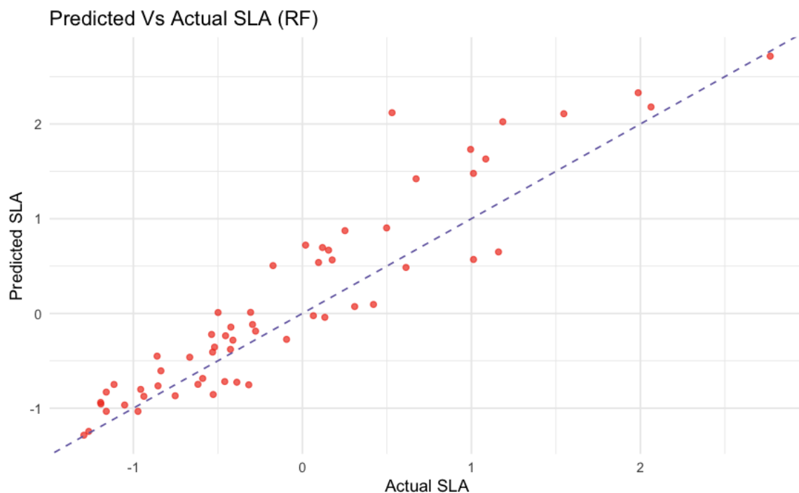
Figure 3.16: The scatter plot created using ggplot2 package, illustrating the predicted and actual SLA values of random forest model
