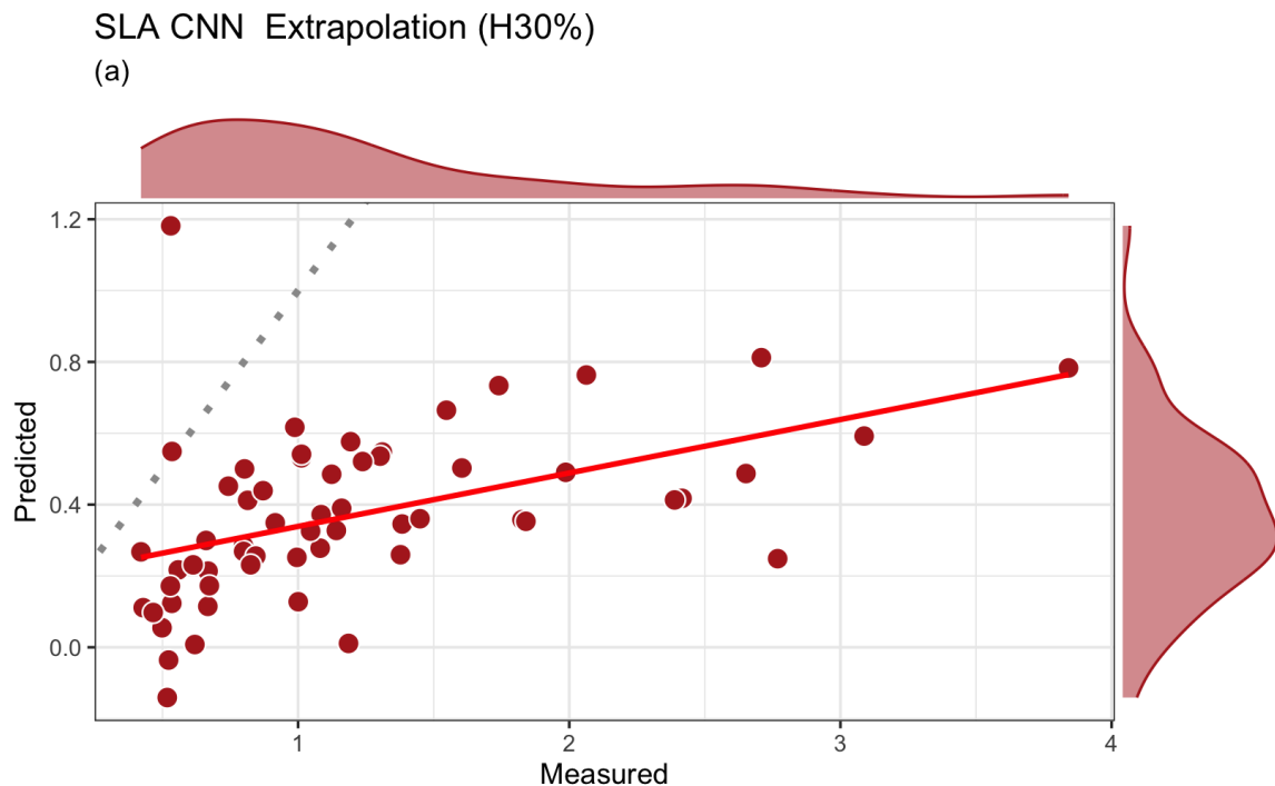
Figure 3.23: The scatter plot illustrates the predicted versus actual SLA values for the extrapolation of the convolutional neural network model on the upper data range. The grey dotted line represents perfect prediction and the red line represents relationship between predicted and measured values based on the linear regression.
