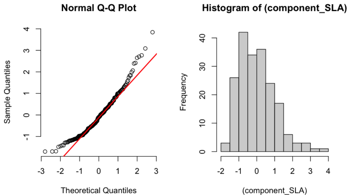
Figure 3.17: Q-Q plot (left) illustrating normality of SLA and histogram (right) showing the distribution of SLA (scaled version) values [15]. The Q-Q plot compares the quantiles of component SLA (Y axis) to the quantile of normal distribution (X axis). Data points closer to the redline has the normal distribution. Deviation from this line indicates the presence of outliers. The histogram shows the frequency of distribution of the scaled SLA values. A perfectly normal distribution will result in a bell shaped histogram.
