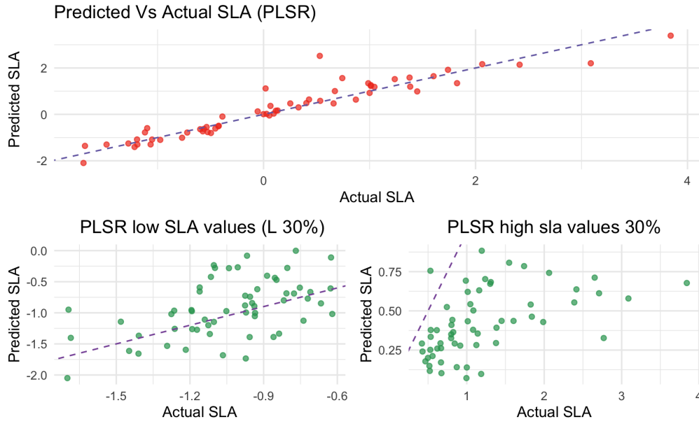
Figure 4.6: This scatter plot presents the extrapolation results as well as the normal PLSR prediction of the SLA trait. It shows the difference in predictive accuracy when tested on higher and lower data ranges.
