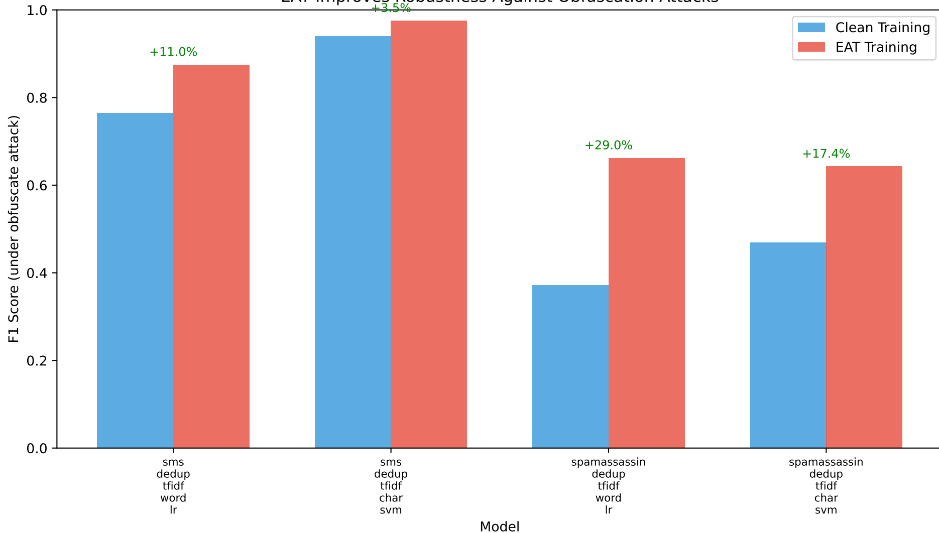
EAT Improves Robustness Against Obfuscation Attacks
