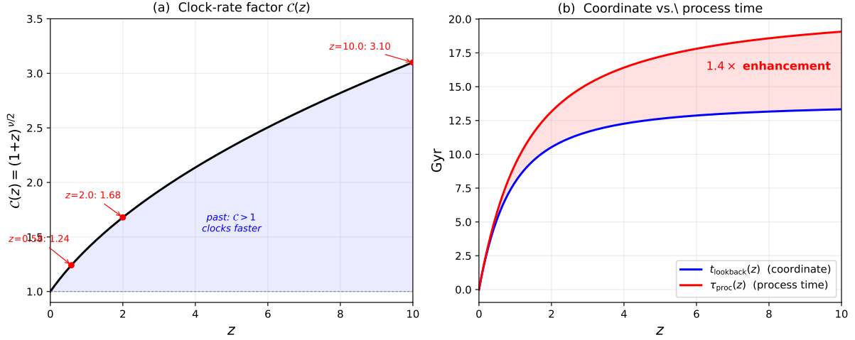
Figure 12: (a) Background history factor C(z) = (1+z)^{\nu/2} with \nu = 0.94 , a power-law approximation calibrated to the companion MOND paper benchmark C(10) \approx 3.1 ; the full C(z) from the coupling-ratio formula (Eq. 368) has a more complex shape at intermediate z . Red dots mark specific benchmarks. (b) Coordinate lookback time (blue) versus cumulative process time (red) from z = 0 to z = 10 . The shaded region is the enhancement due to the faster process-clock rate in the past. Both panels use standard \Lambda CDM H(z) with \Omega_m = 0.315 , H_0 = 67.4 \text{ km s}^{-1} \text{ Mpc}^{-1} .
