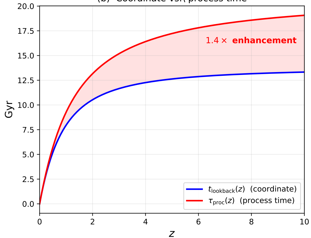
(b) Coordinate vs. process time
