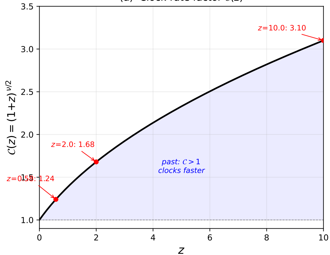
(a) Clock-rate factor C(z)
