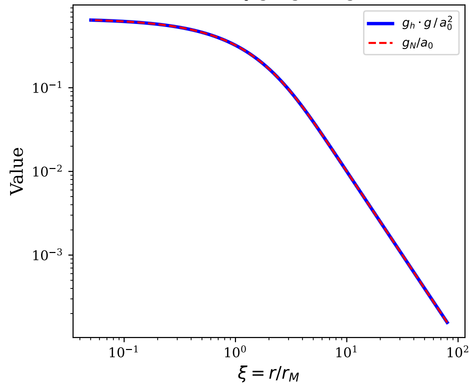
(a) Verify g_h \cdot g = a_0 g_N
