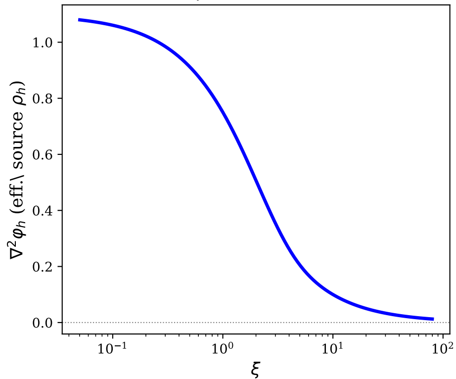
(b) \rho_h \geq 0 at all radii
