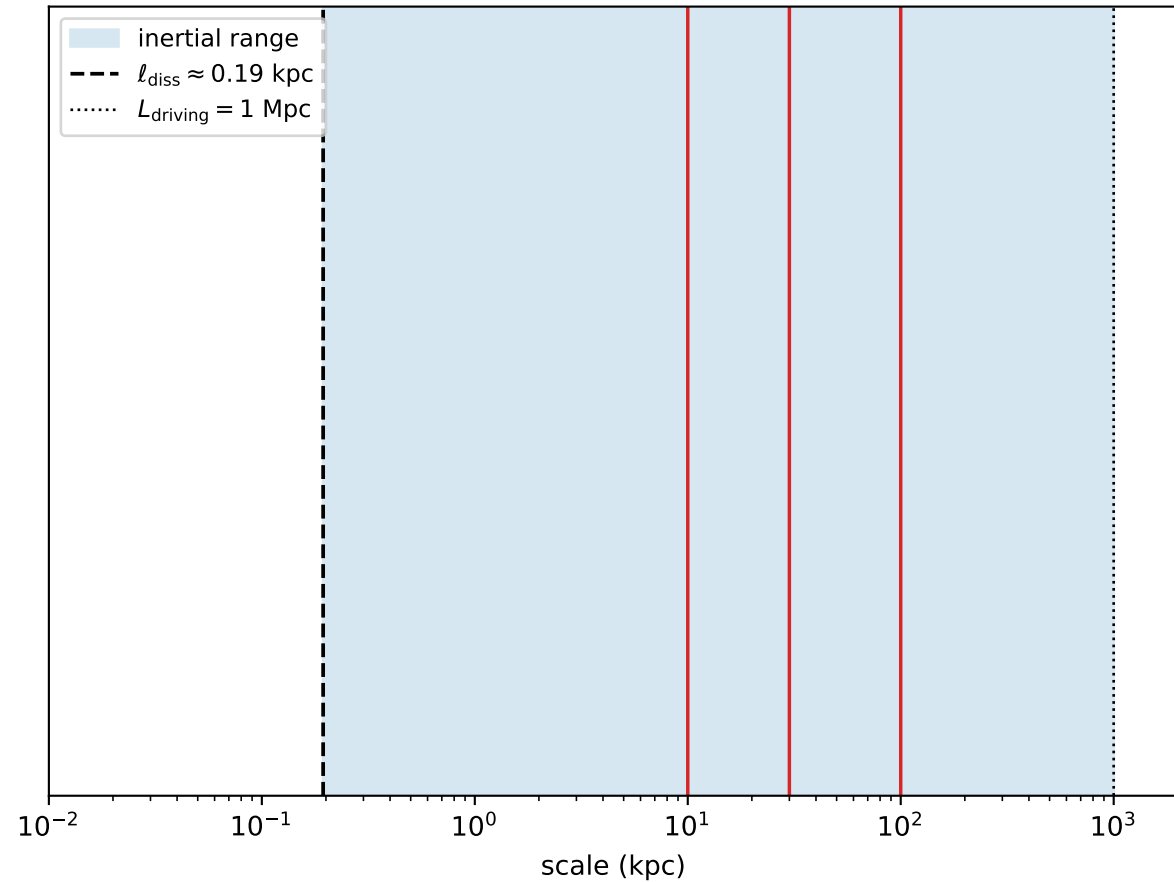
Conservative cascade window ( \text{Re}_{\text{min}} \approx 8.90\text{e} + 04 )
