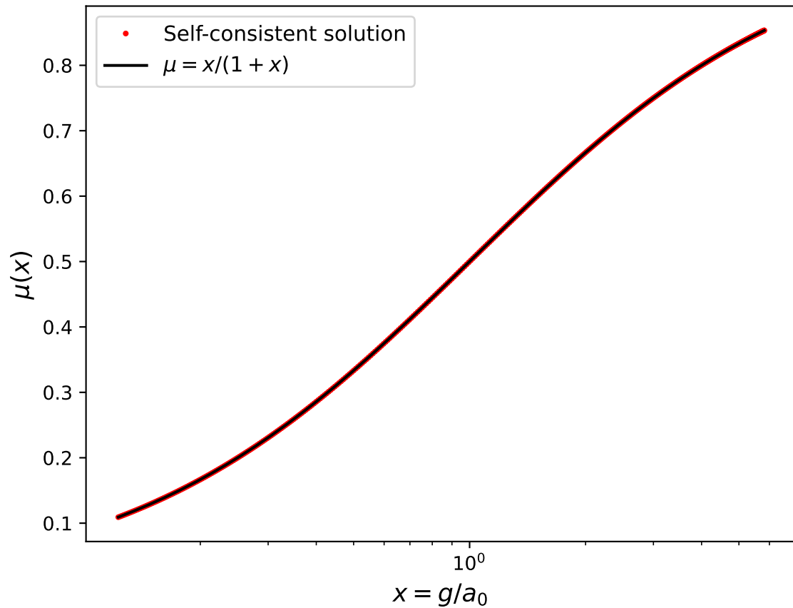
\mu(x) from self-consistent equation
