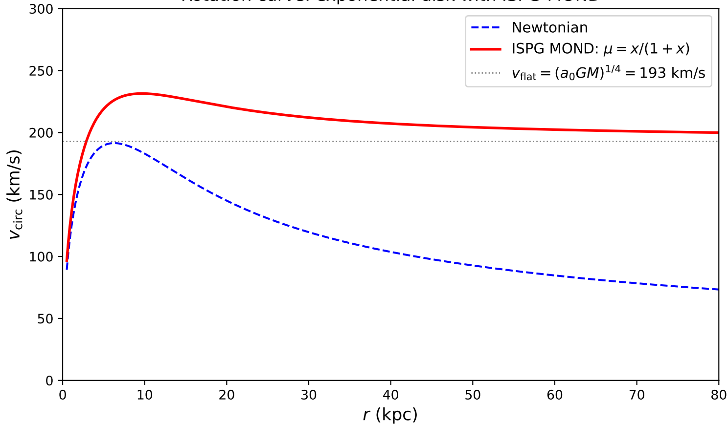
Rotation curve: exponential disk with ISPG-MOND
