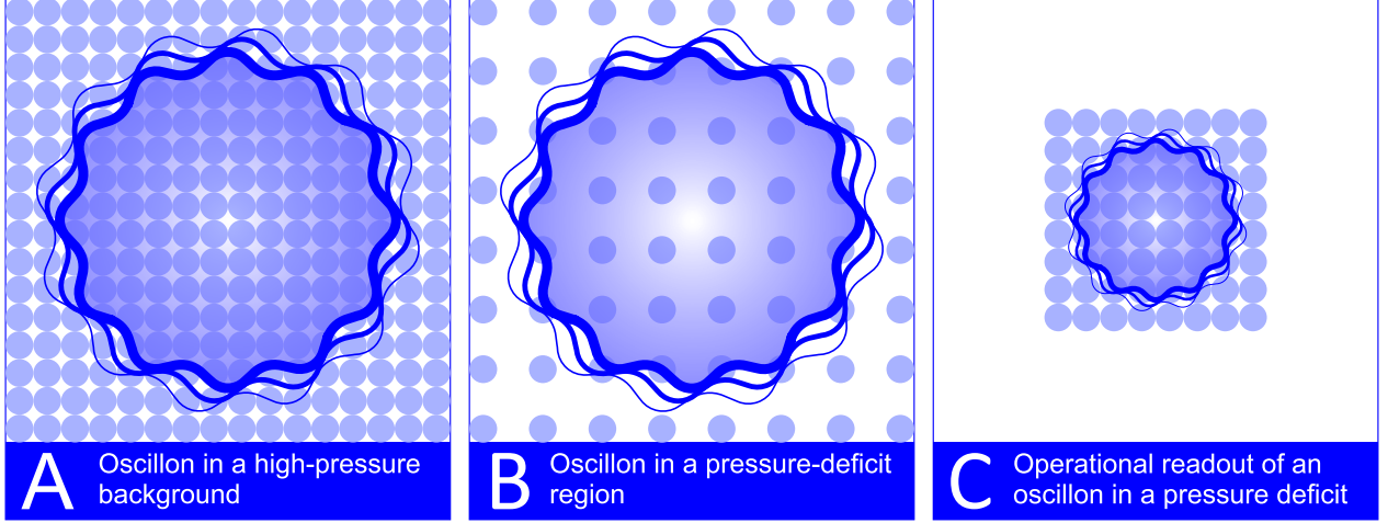
Figure 1: Operational readout of an oscillon within a pressure-deficit zone. (A) In an unperturbed foundation-medium whose pressure is higher than in the deficit zone, an oscillon occupies a comparatively dense nodal arrangement; inter-node coupling is stronger and local processes proceed at a higher coordinate cadence. (B) Within a pressure-deficit zone, foundation nodes are rarefied; operational inter-node separation increases, transmission cadence falls, and the local passage of time slows. (C) In external readout, an oscillon within a pressure deficit is registered with a slower clock cadence, smaller operational size, and changed effective mass; the increased internal interval does not enter as an independently measurable quantity.
