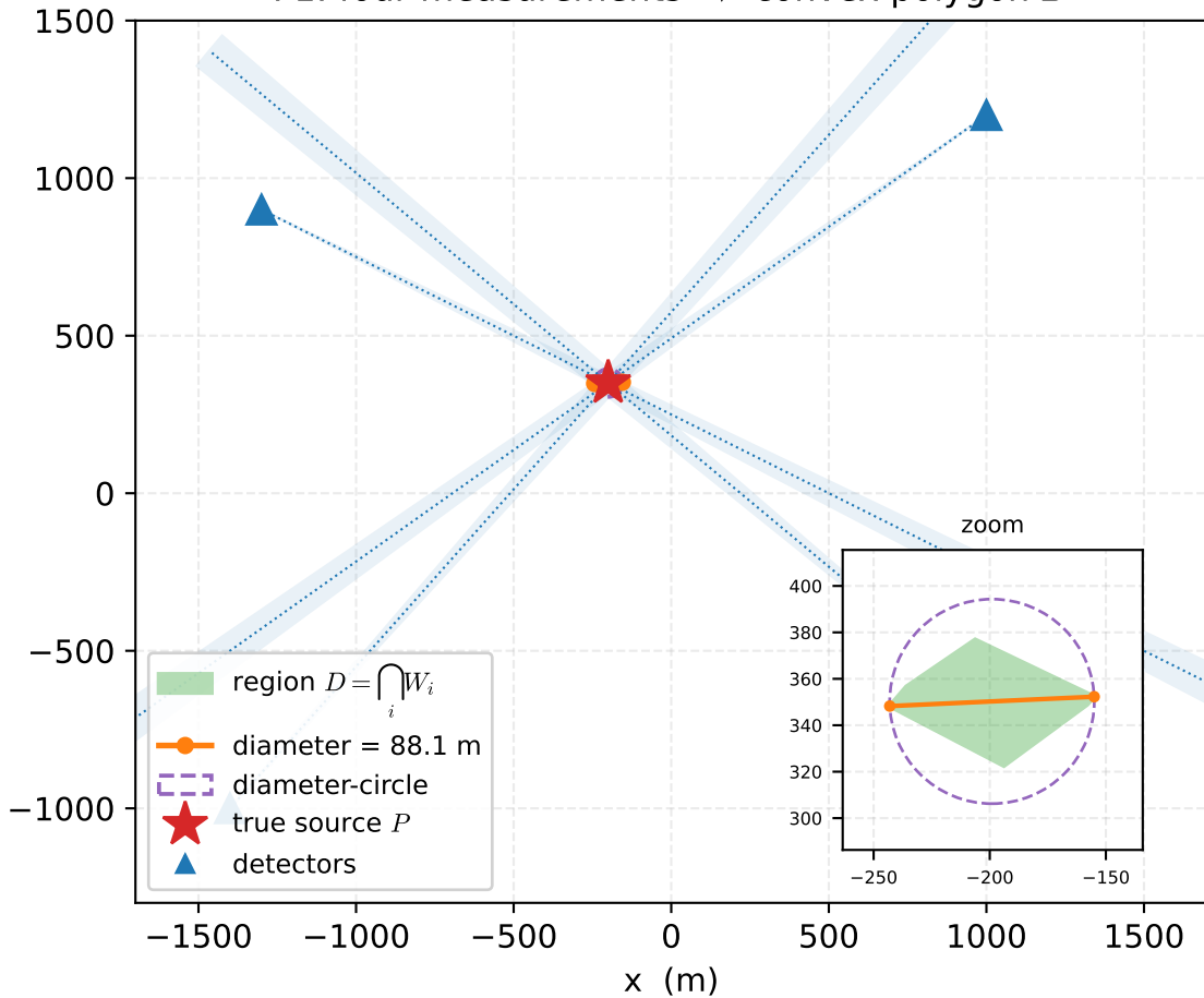
P1: four measurements \Rightarrow convex polygon D
