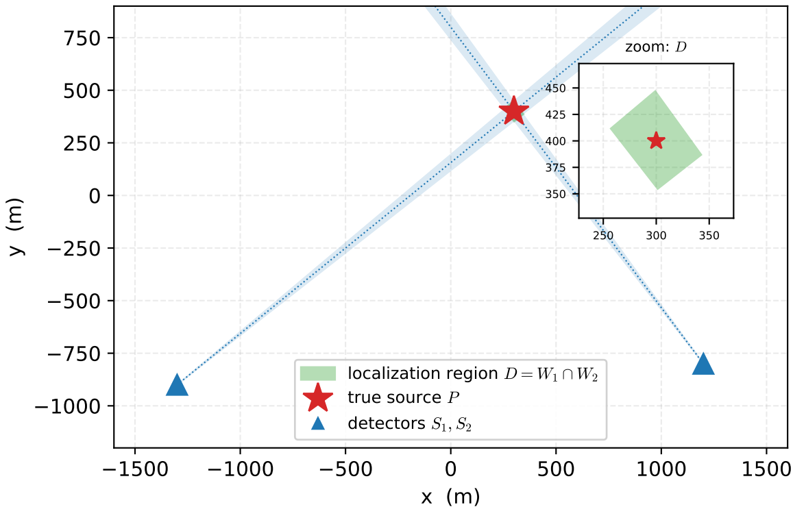
P1: two wedges intersect to a small region (diam \approx 90.7 m)
