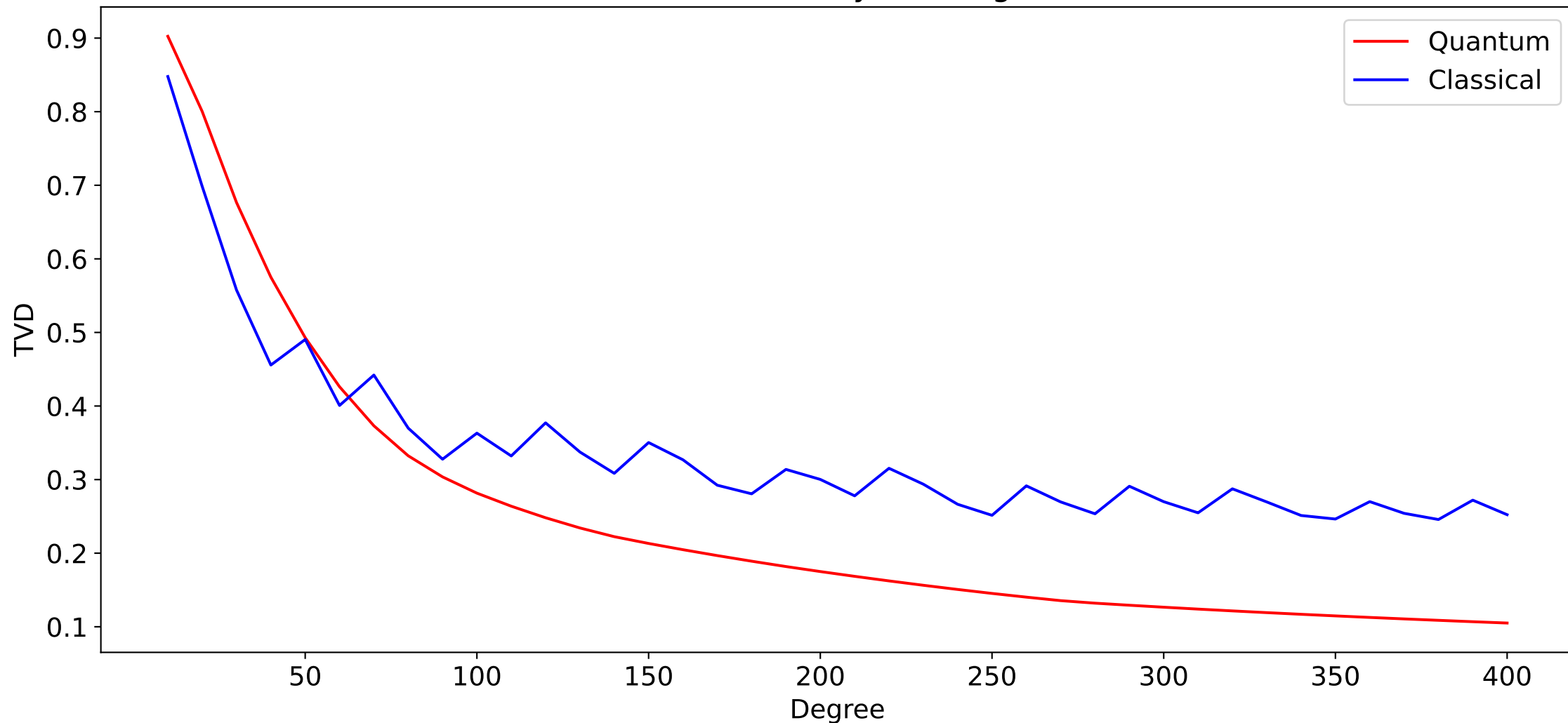
Simulations of a Dyson Ising Chain
