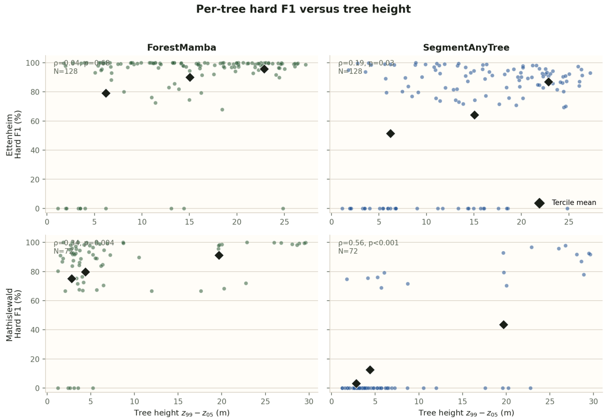
Figure 20: Per-tree hard F1 against tree height ( z_{99} - z_{05} ) for ForestMamba and SegmentAnyTree at Ettenheim (top) and Mathisleswald (bottom). Diamonds are tercile means.
