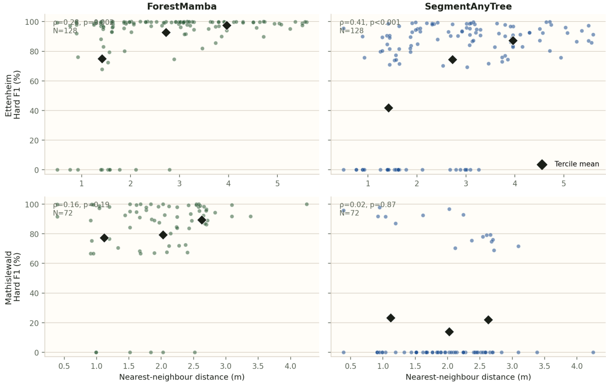
Figure 21: Per-tree hard F1 against planimetric nearest-neighbour distance for ForestMamba and SegmentAnyTree at Ettenheim (top) and Mathislewald (bottom). Diamonds are tercile means.
