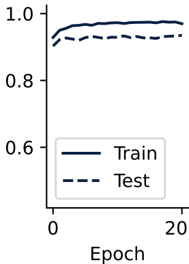
Accuracy
