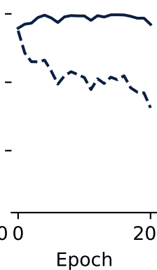
Recall
