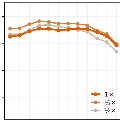
BirdAVES
