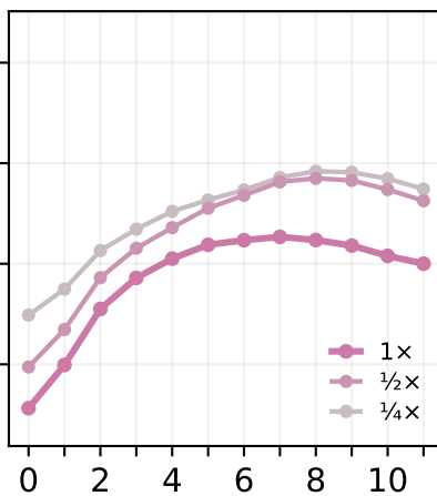
BEATs
