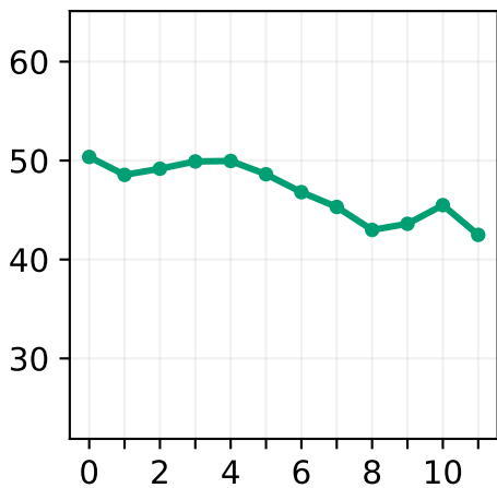
HuBERT
