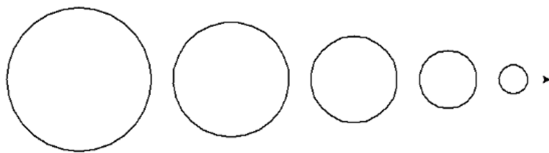
Figure 3: Turtle Circles 2
