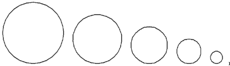
Figure 2: Turtle Circles 1
