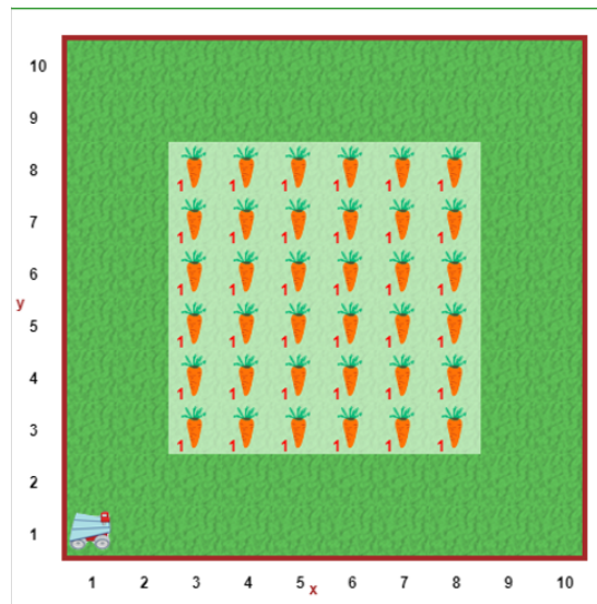
Figure 6: Reeborg Carrots
