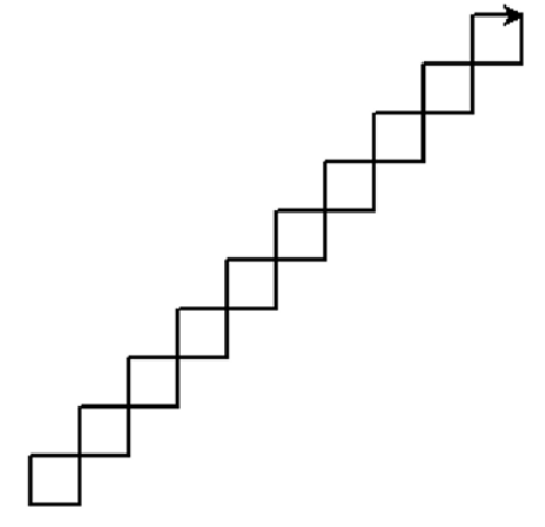
Figure 7: Turtle Stairs
