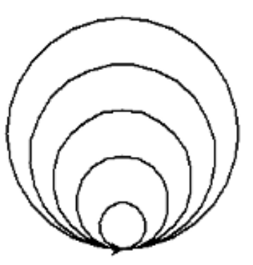
Figure 4: Turtle Circles 3
