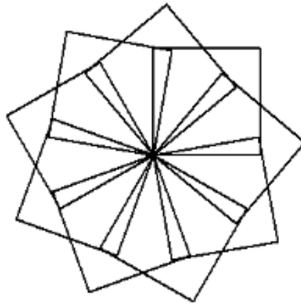
Figure 5: Turtle Star
