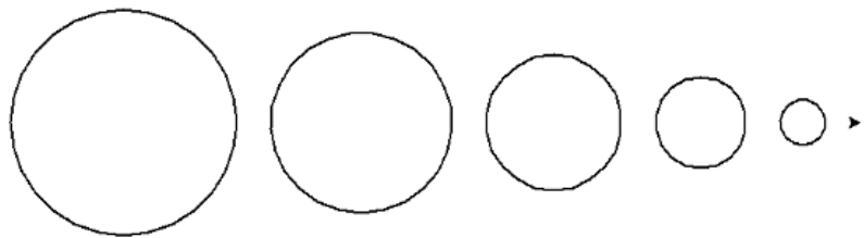
Figure 3: Turtle Circles 2
