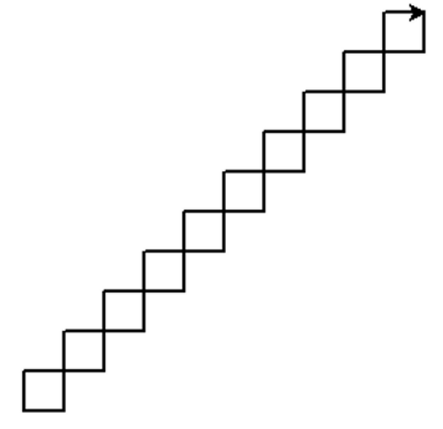
Figure 7: Turtle Stairs
