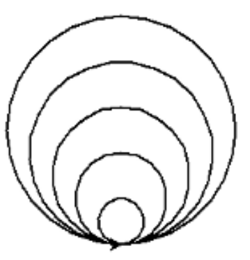
Figure 4: Turtle Circles 3
