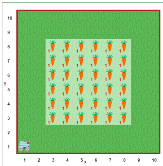
Figure 6: Reeborg Carrots
